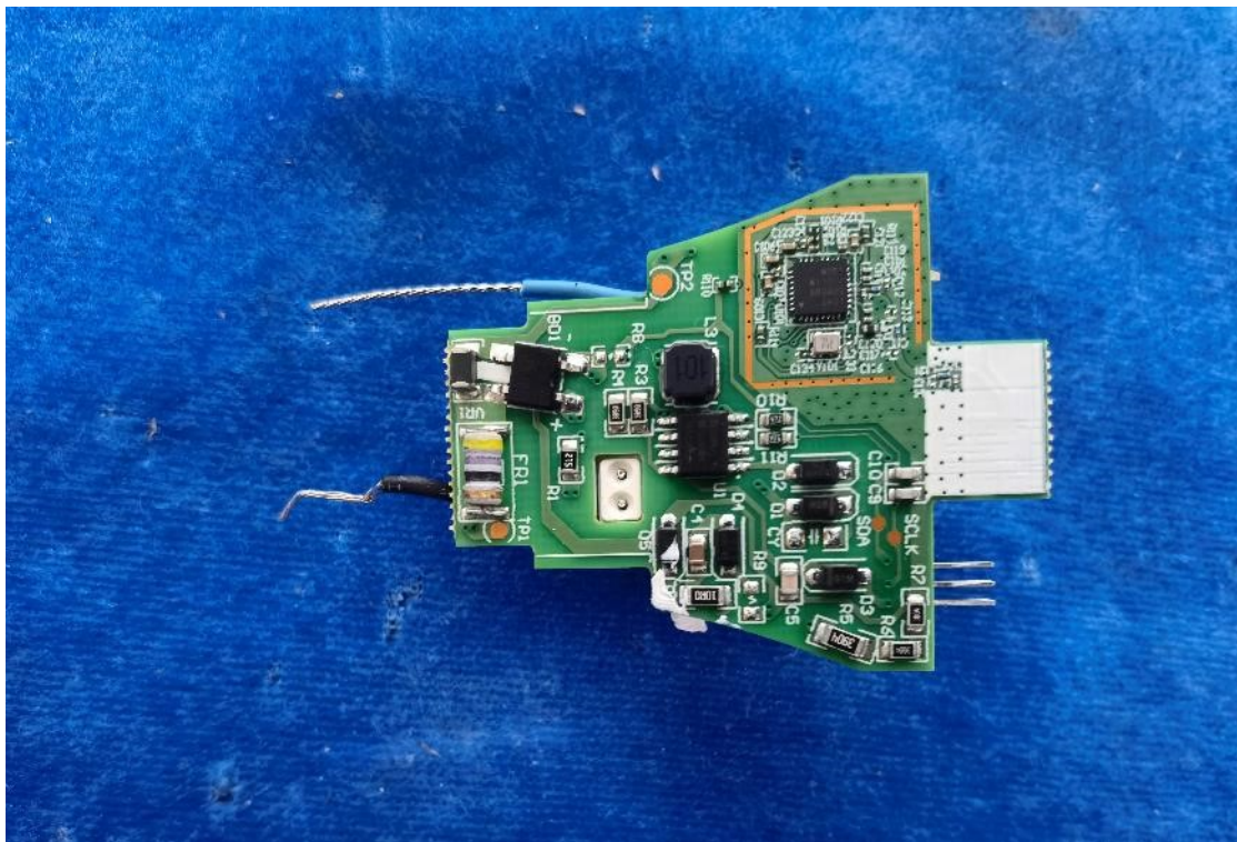
PCB (with SILAB RF IC))
