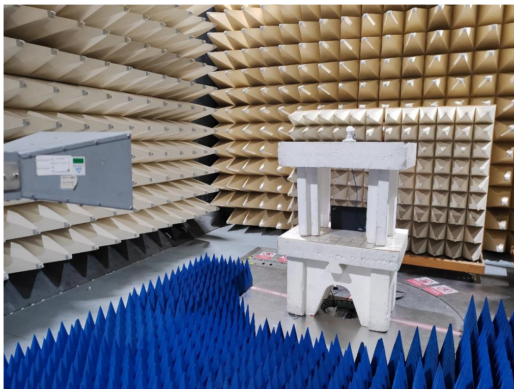
Photograph 4: Set-up photo for Radiated Emission, 1GHz - 18GHz
