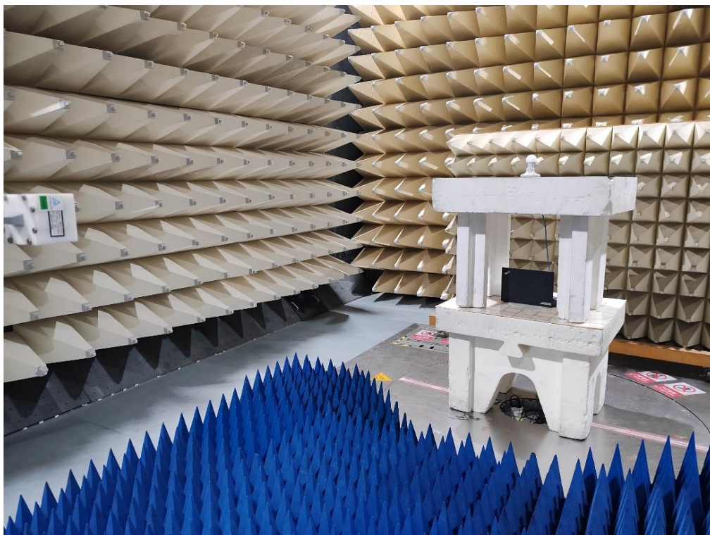
Photograph 5: Set-up photo for Radiated Emission, 18GHz - 25GHz
