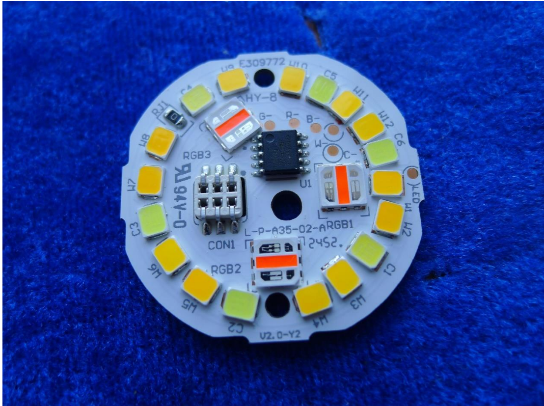
LED Module
