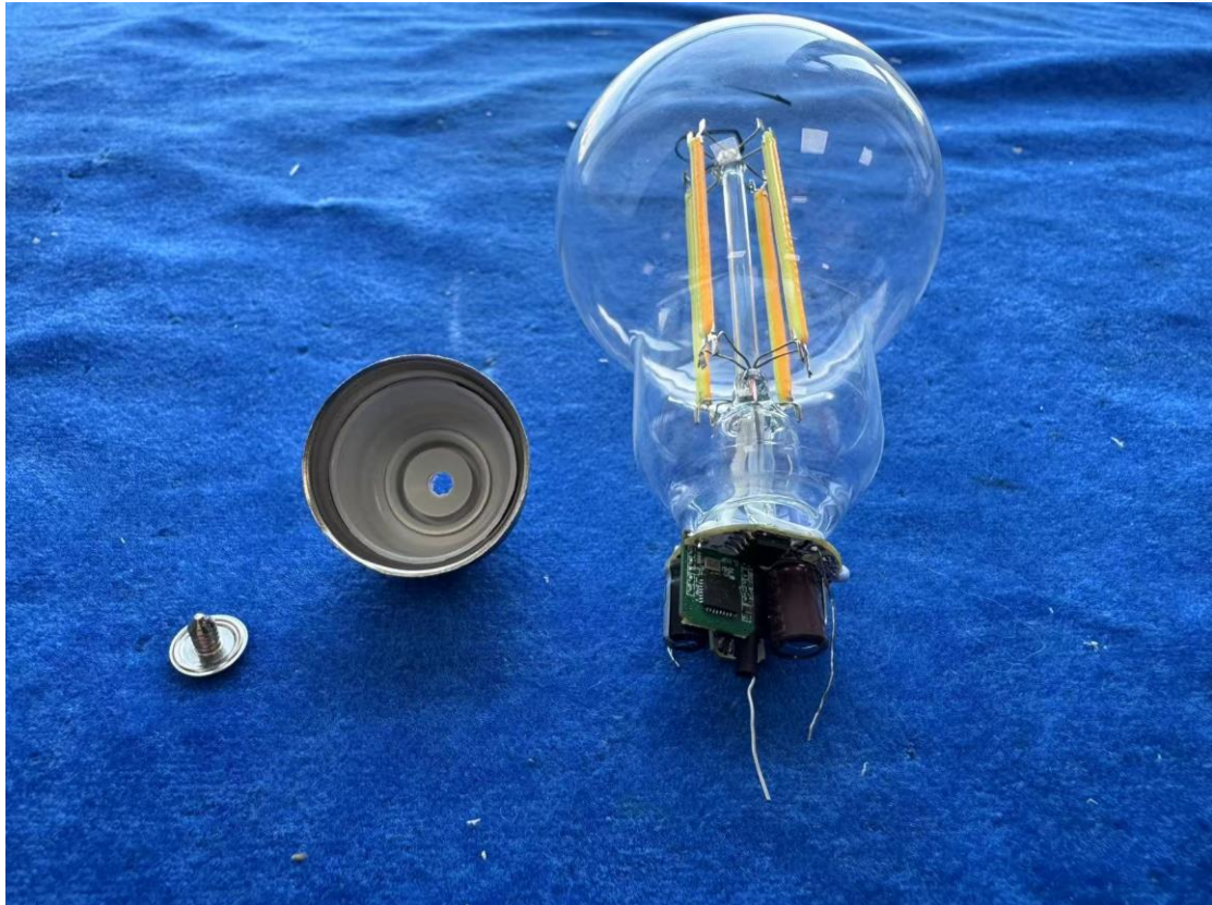
Internal View (with SILAB RF IC)
