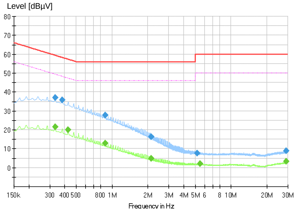
Figure 2: Spectral Diagrams, Conducted Emission, 150 kHz – 30 MHz, N line
