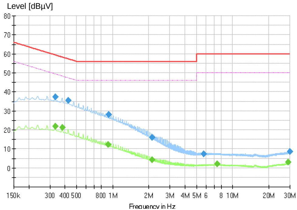
Figure 1: Spectral Diagrams, Conducted Emission, 150 kHz – 30 MHz, L line
