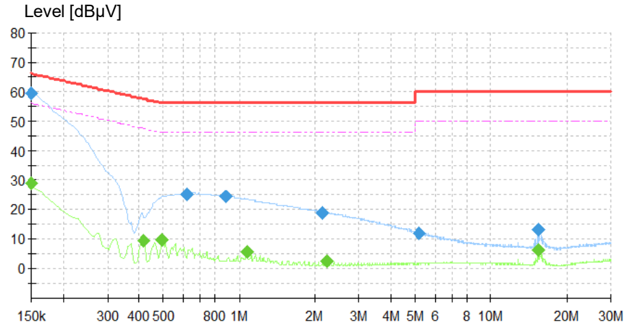
Figure 3: Spectral Diagrams, Conducted Emission, 150 kHz – 30 MHz, L, Mode 2
