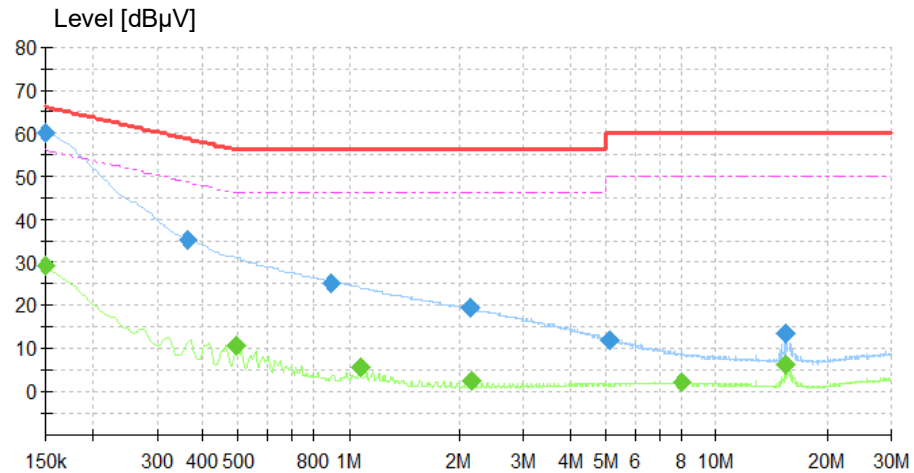
Figure 4: Spectral Diagrams, Conducted Emission, 150 kHz – 30 MHz, N, Mode 2
