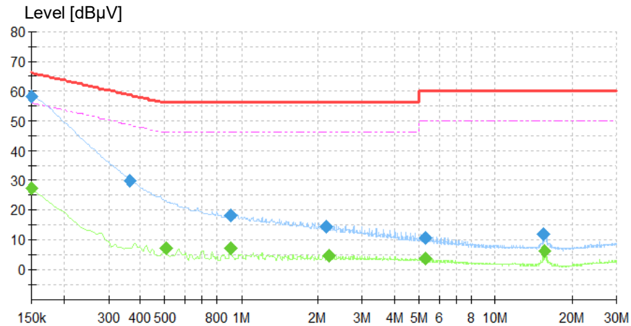
Figure 1: Spectral Diagrams, Conducted Emission, 150 kHz – 30 MHz, L, Mode 1
