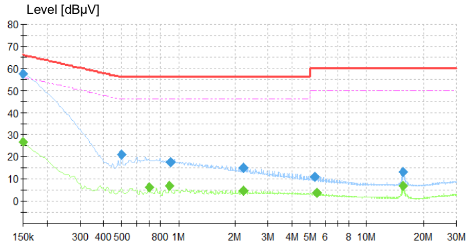
Figure 2: Spectral Diagrams, Conducted Emission, 150 kHz – 30 MHz, N, Mode 1
