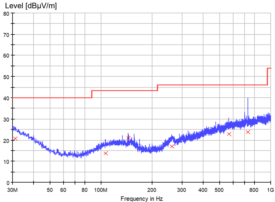
Figure 3: Spectral Diagrams, Radiated Emission, 30 MHz – 1000 MHz, Horizontal polarization on mode 1
