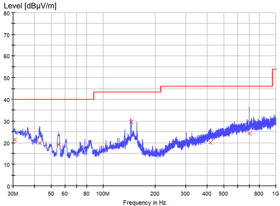
Figure 4: Spectral Diagrams, Radiated Emission, 30 MHz – 1000 MHz, Vertical polarization on mode 1
