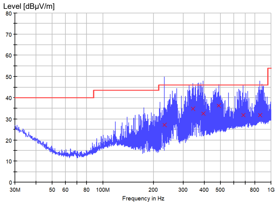
Figure 7: Spectral Diagrams, Radiated Emission, 30 MHz – 1000 MHz, Horizontal polarization on mode 3
