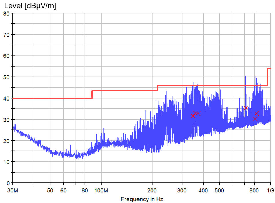
Figure 5: Spectral Diagrams, Radiated Emission, 30 MHz – 1000 MHz, Horizontal polarization on mode 2
