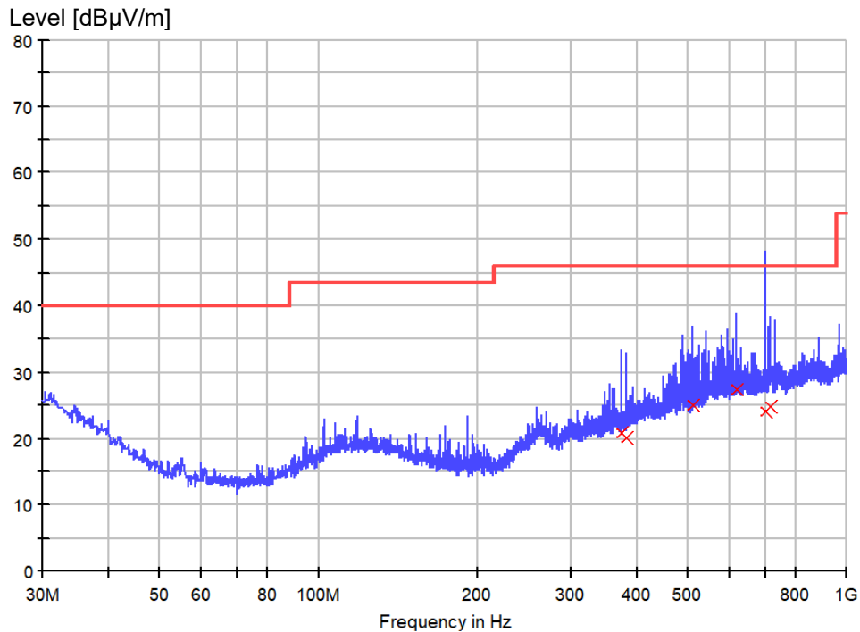
Figure 6: Spectral Diagrams, Radiated Emission, 30 MHz – 1000 MHz, Vertical polarization on mode 2
