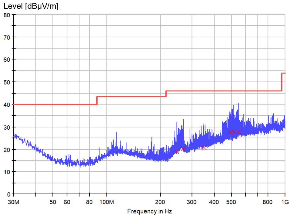
Figure 8: Spectral Diagrams, Radiated Emission, 30 MHz – 1000 MHz, Vertical polarization on mode 3
