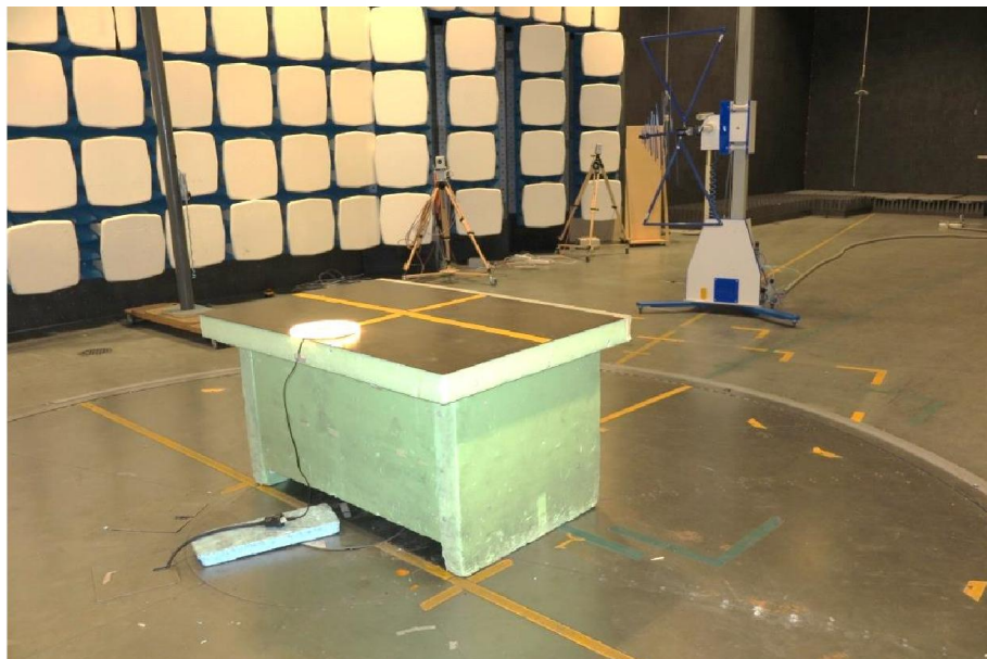
Test set up radiated emission 30 MHz – 1 GHz
