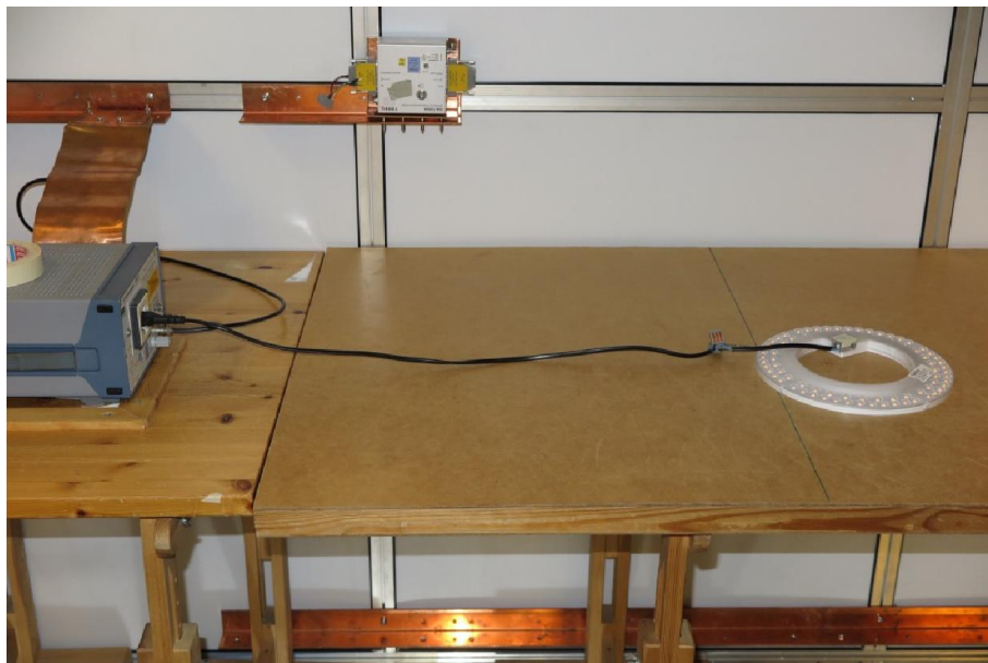
Test setup for conducted emission 150 kHz – 30 MHz
