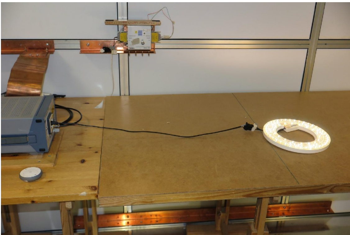
Test setup for conducted emission 150 kHz – 30 MHz
