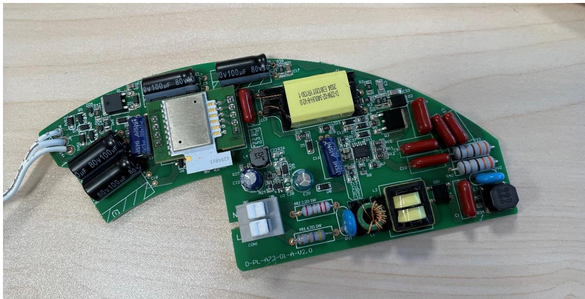
PCB BACK VIEW
