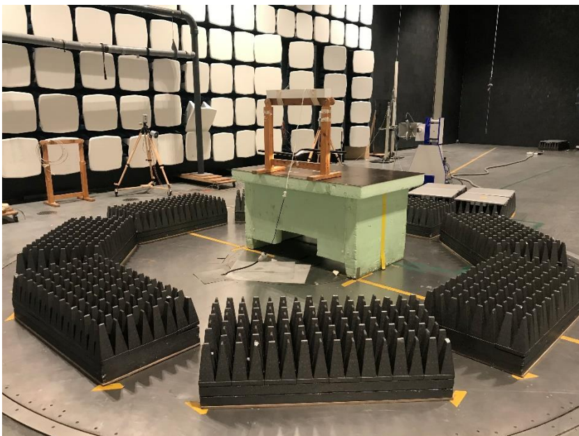
Test set up radiated emission 1 - 13 GHz
