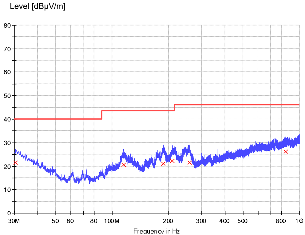
Figure 5: Spectral Diagrams, Radiated Emission, 30 MHz – 1000 MHz, Horizontal polarization on mode 1
