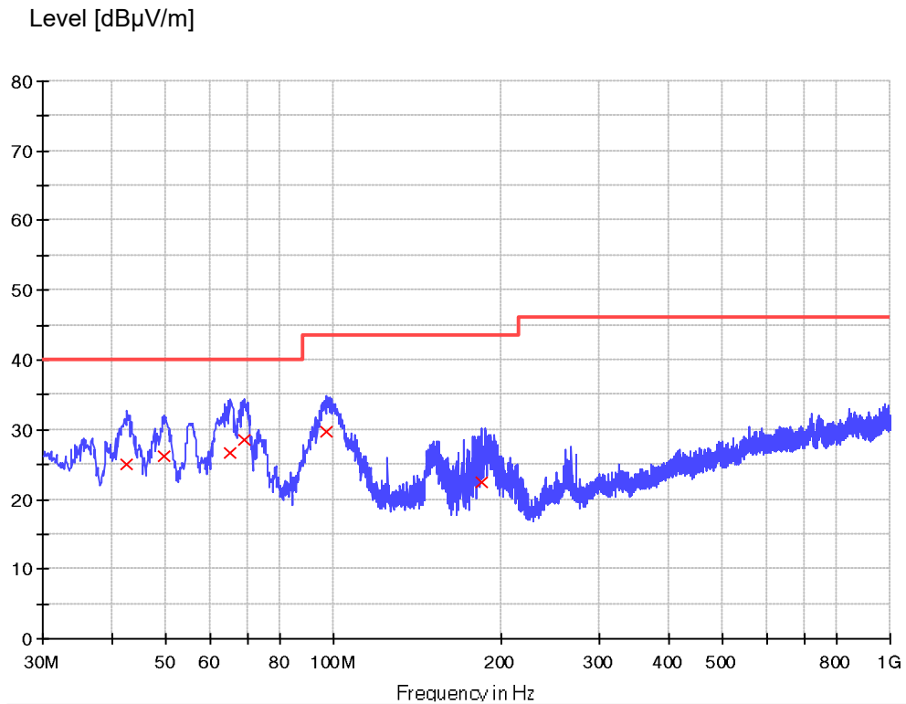
Figure 8: Spectral Diagrams, Radiated Emission, 30 MHz – 1000 MHz, Vertical polarization on mode 2
