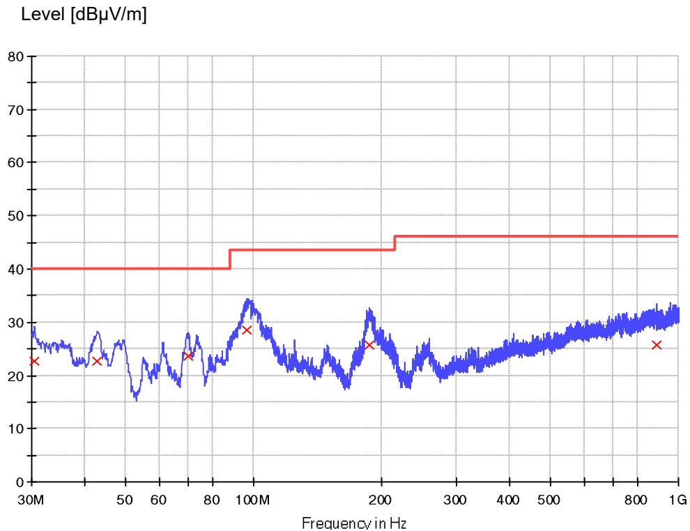
Figure 6: Spectral Diagrams, Radiated Emission, 30 MHz – 1000 MHz, Vertical polarization on mode 1
