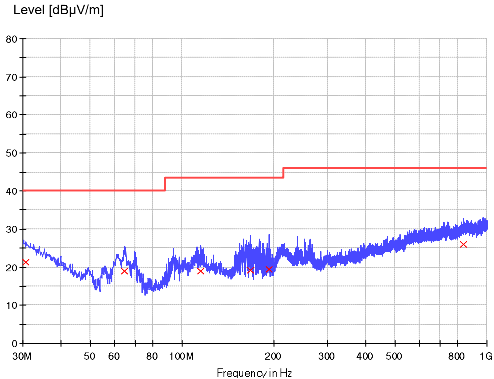
Figure 7: Spectral Diagrams, Radiated Emission, 30 MHz – 1000 MHz, Horizontal polarization on mode 2
