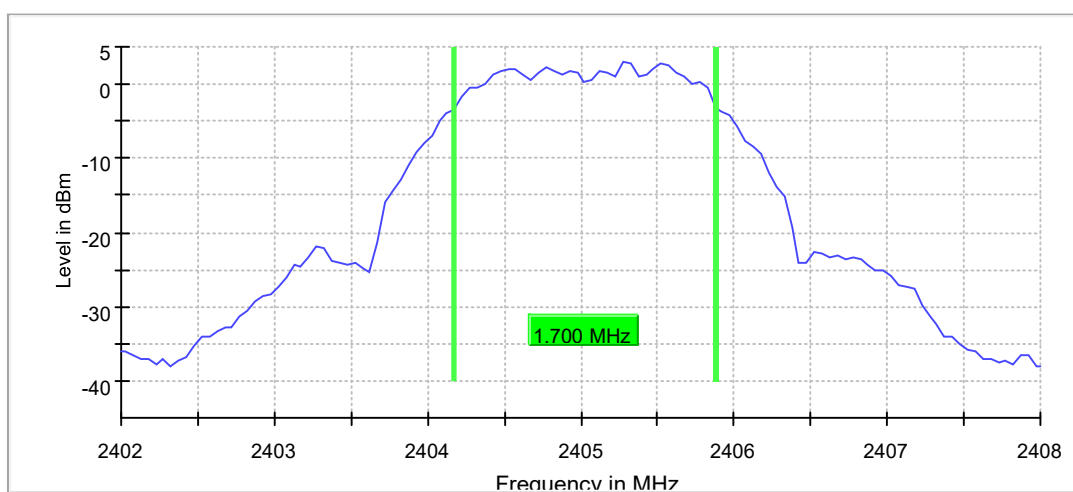
6 dB Bandwidth
