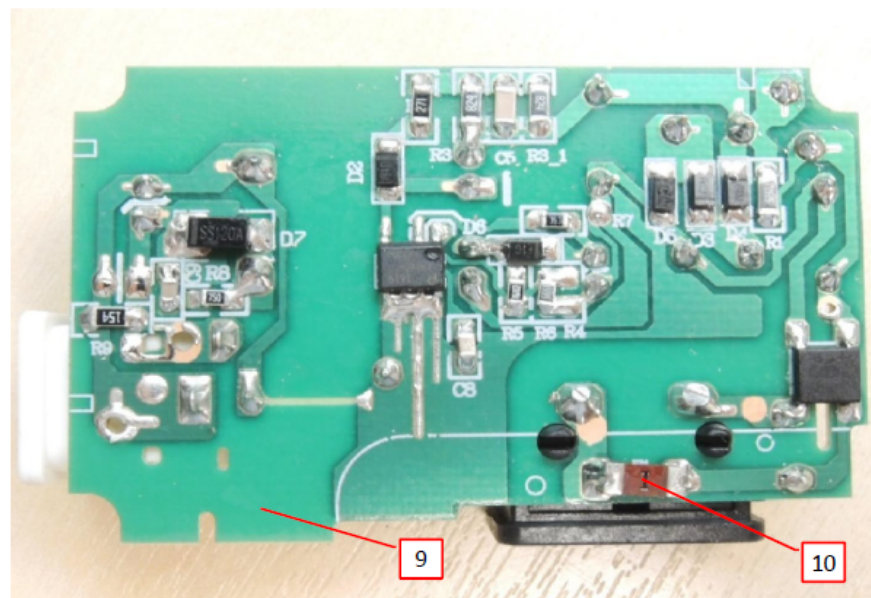
Photo 8 -External view of PWB rear side
