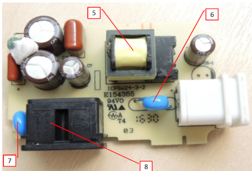
Photo 8 -External view of PWB rear side
