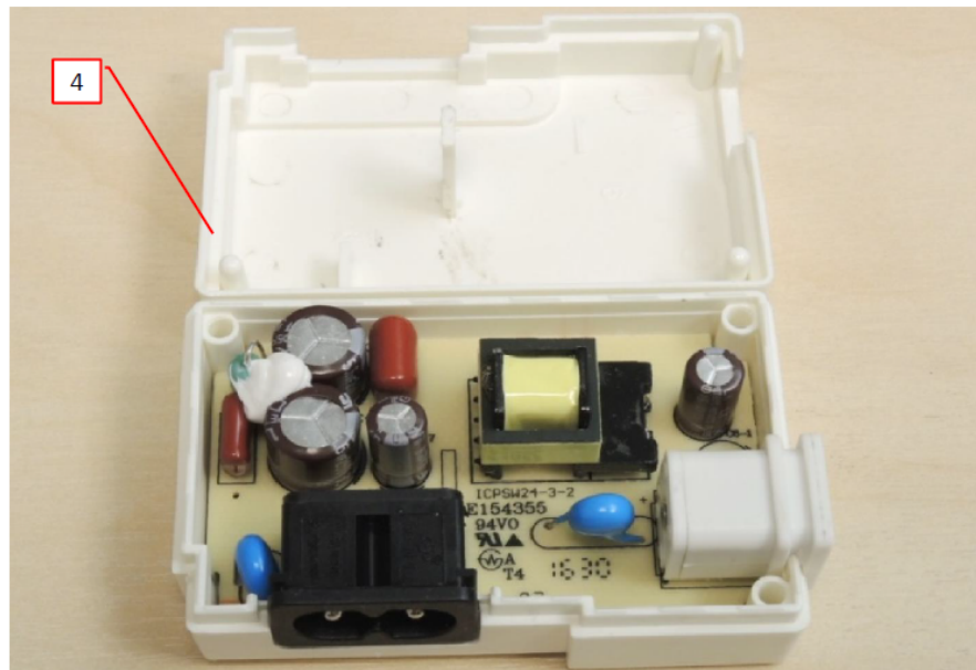
Photo 7 -External view of the PWB component side
