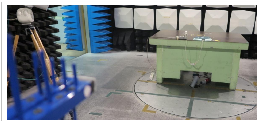
Test set up radiated emission 30 MHz – 1 GHz
