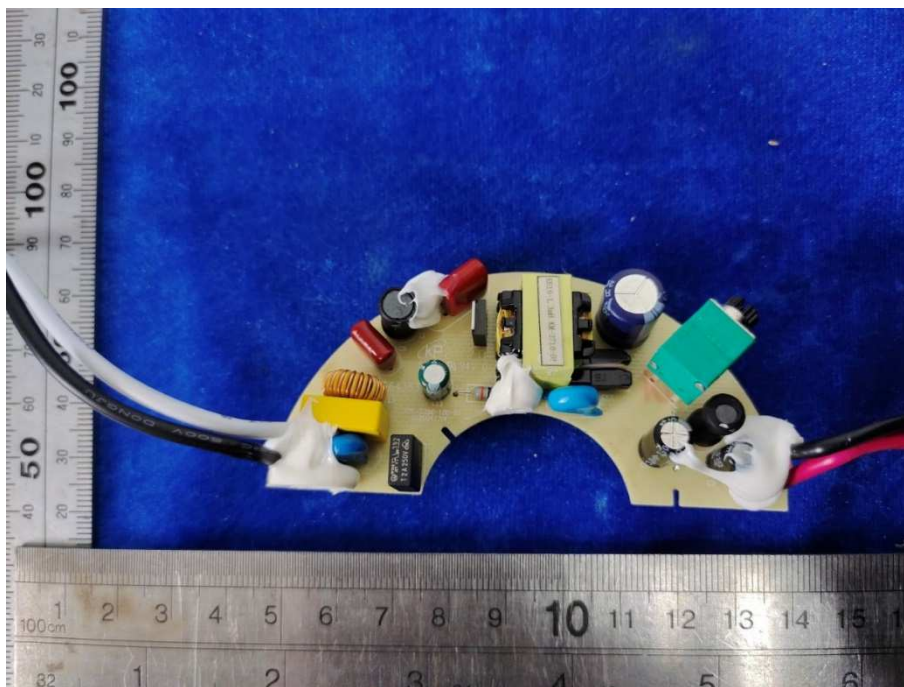
LED driver View
