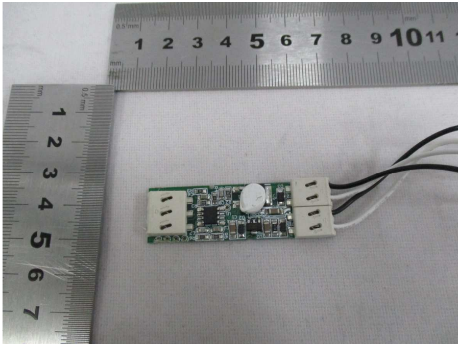
Dimmer PCB
