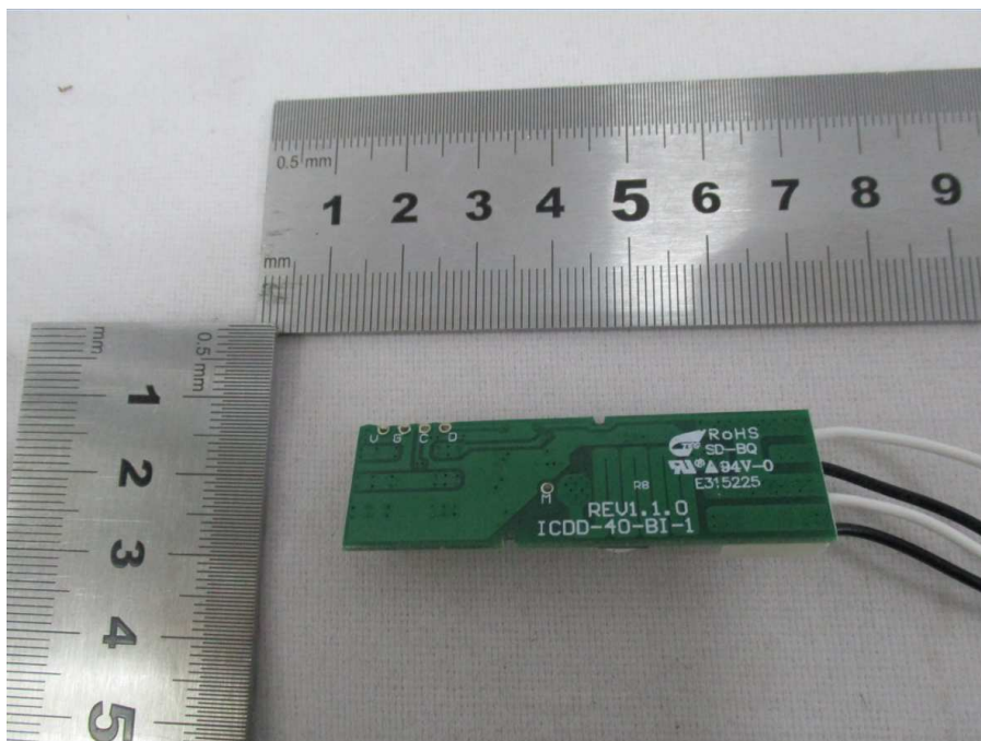
Dimmer PCB
