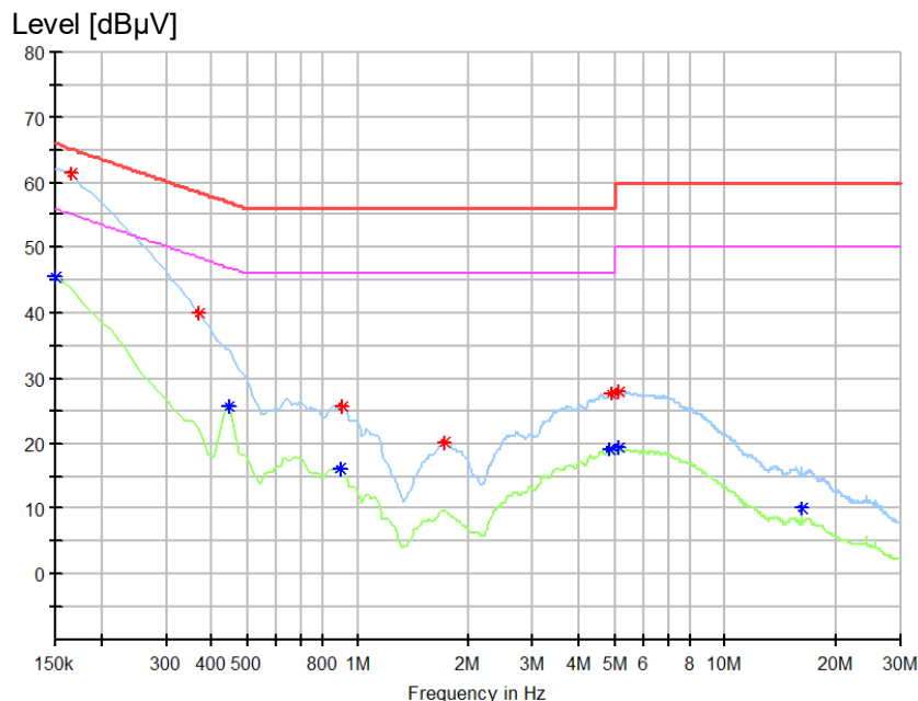
Figure 2: Spectral Diagrams, Conducted Emission, 150 kHz – 30 MHz, N
