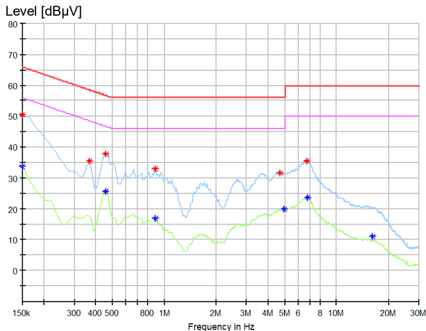
Figure 1: Spectral Diagrams, Conducted Emission, 150 kHz – 30 MHz, L
