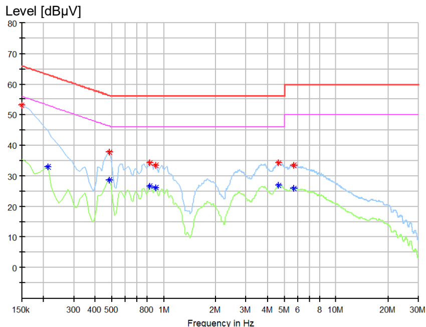
Figure 1: Spectral Diagrams, Conducted Emission, 150 kHz – 30 MHz, L
