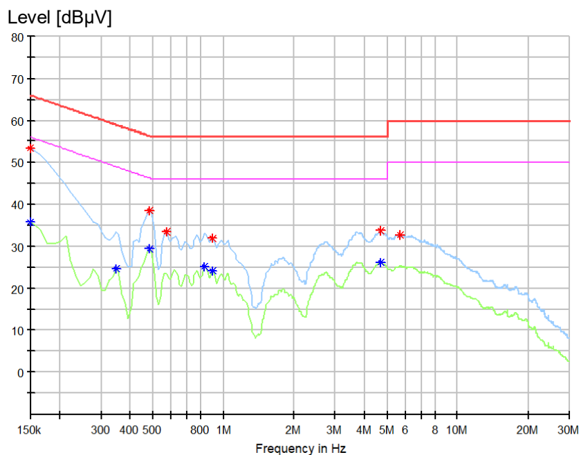
Figure 2: Spectral Diagrams, Conducted Emission, 150 kHz – 30 MHz, N
