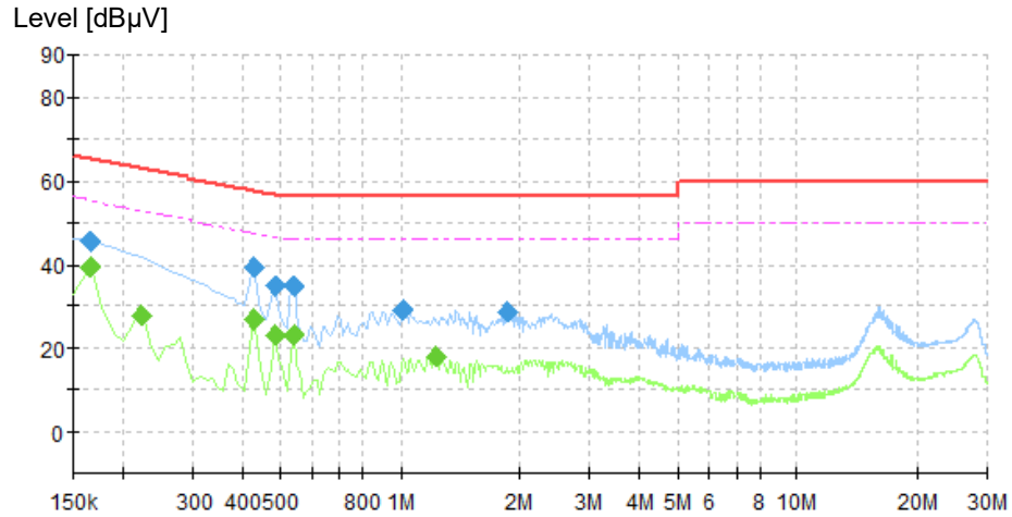
Figure 2: Spectral Diagrams, Conducted Emission, 150 kHz – 30 MHz, N
