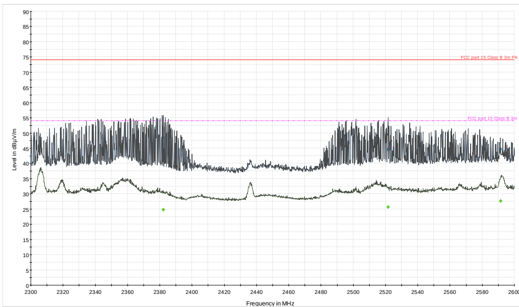
Diagram, band edge overview, with filter correction in the 2.4 -2.5 GHz band.
