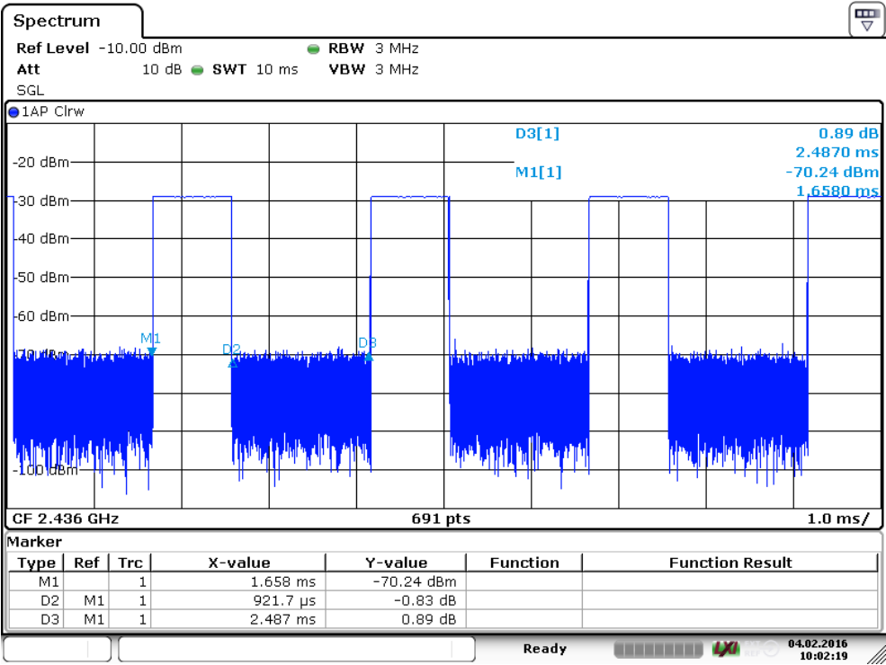
Screenshot: Duty cycle measurement
