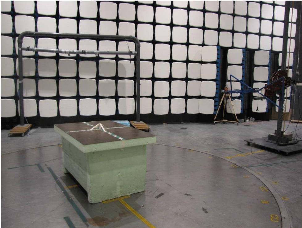
Test set up radiated emission 1GHz – 13 GHz
