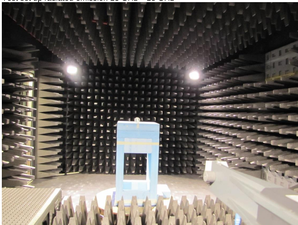
Test set up radiated emission 18 GHz – 26 GHz
