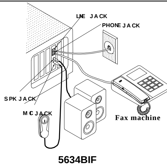
Figure 1-5. Completed modem installation
