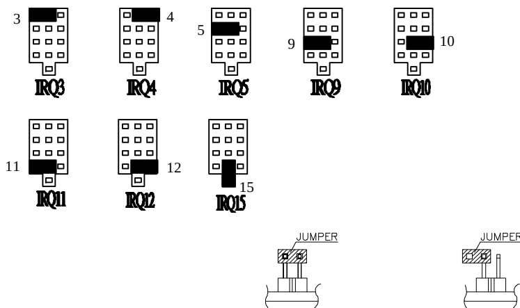
Figure 1-2. Jumper diagram
