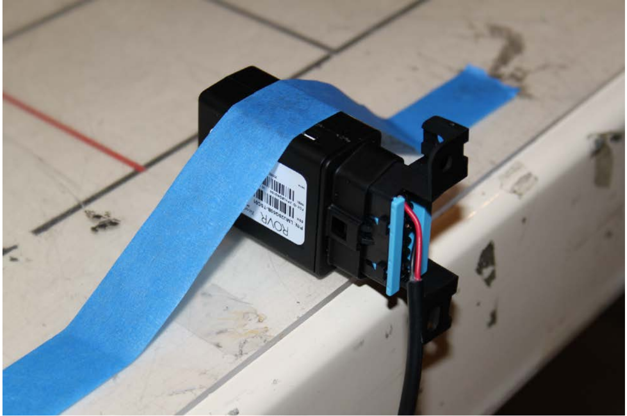
Radiated Emissions Test Setup (all axes verified)
