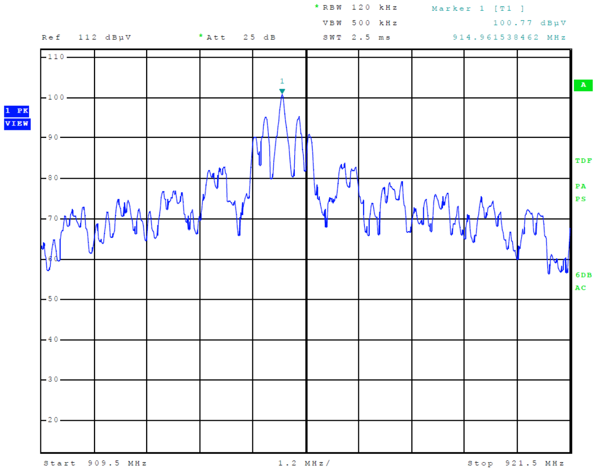
Figure 1 Transmitter Output Across Frequency Band – IAG Boost
