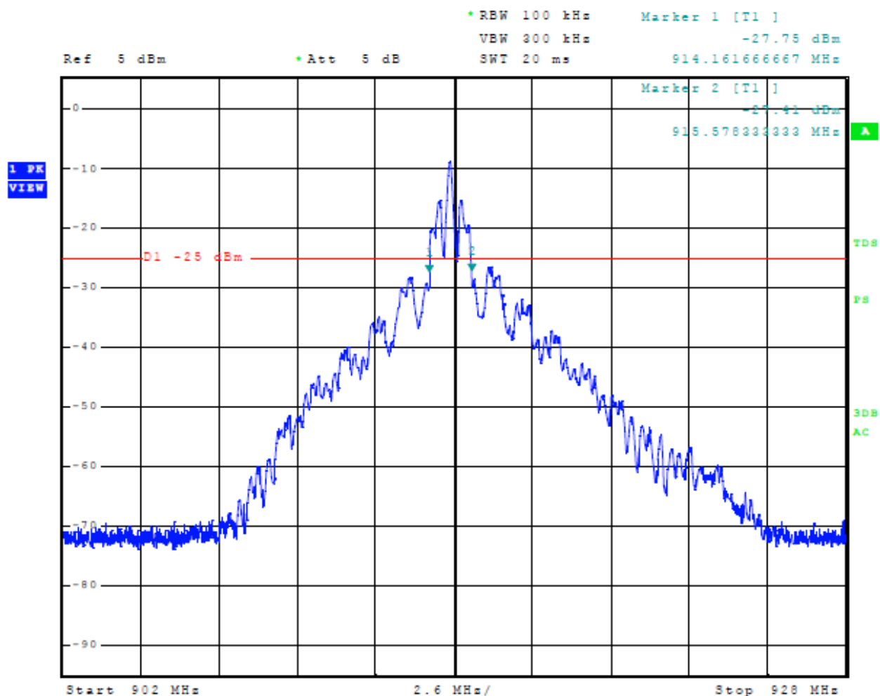
Figure 3 Emissions Mask
