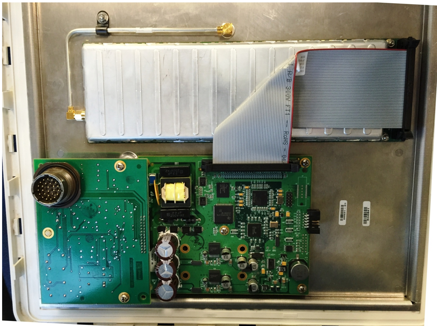
1. E4H Overview Photo
