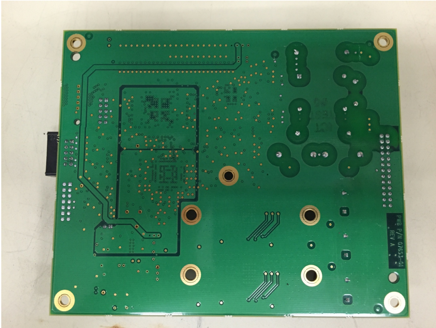
7. E4H - DSP/Power Supply Board, Back Side
