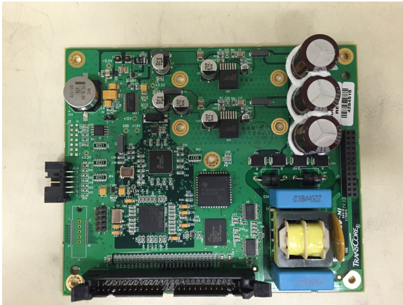
6. E4H - DSP/Power Supply Board, Component Side (FIH-05939)
