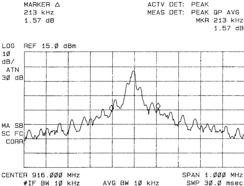
Figure 5 Occupied Bandwidth Modulated Mode
