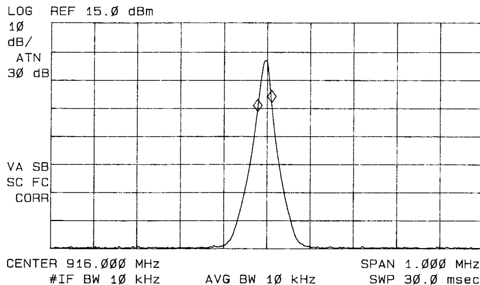
Figure 4 Occupied Bandwidth CW Mode
