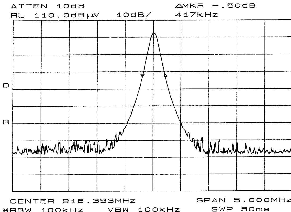
Figure 1 99.5% Power Occupied Bandwidth
