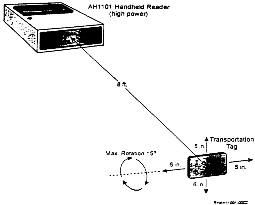
Figure 3-5 Distance and Orientation for Correctly Reading a Tag Using the High-Power Handheld Reader
