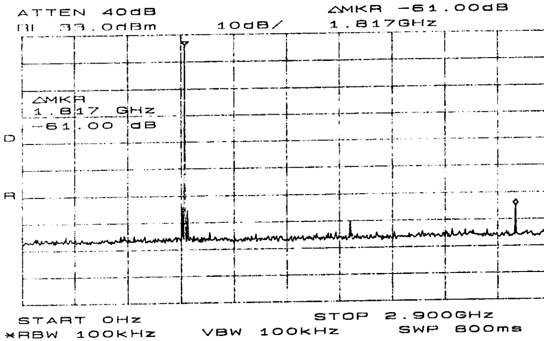
Plot 5 Spurious Emissions at Antenna Terminal Low Power
