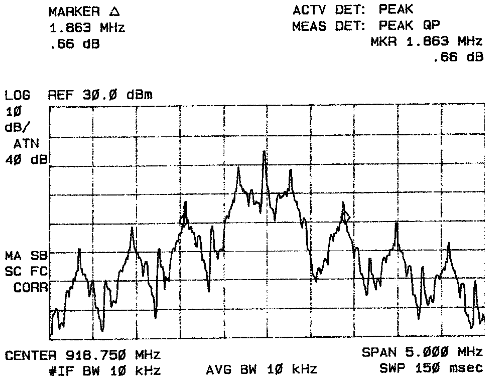
Figure 9 Occupied Bandwidth Modulated 918.75 MHz
