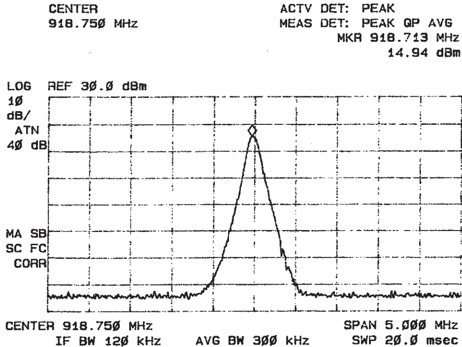
Figure 4 6dB Attenuation @ 918.75 MHz
