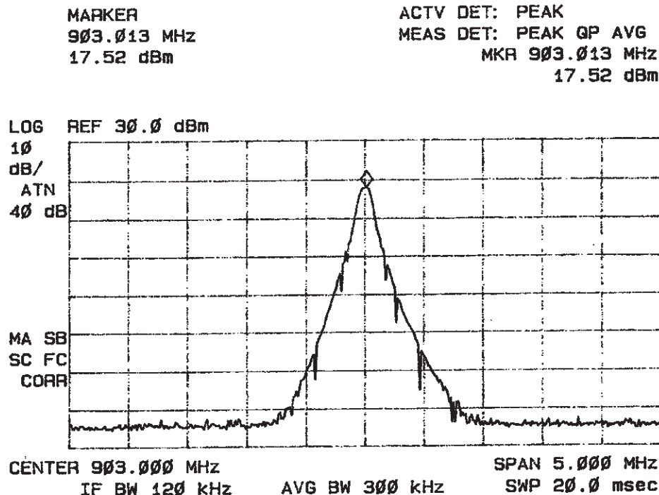
Figure 3 6dB Attenuation @ 903.0 MHz
