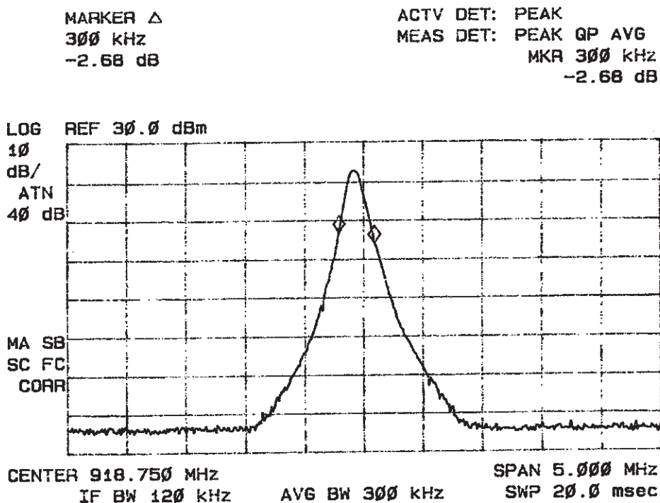
Figure 8 Occupied Bandwidth CW Mode 918.75 MHz
