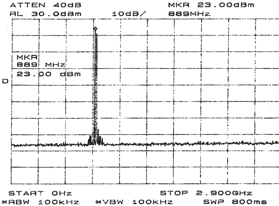
Figure 10 Emissions at Antenna Terminal
