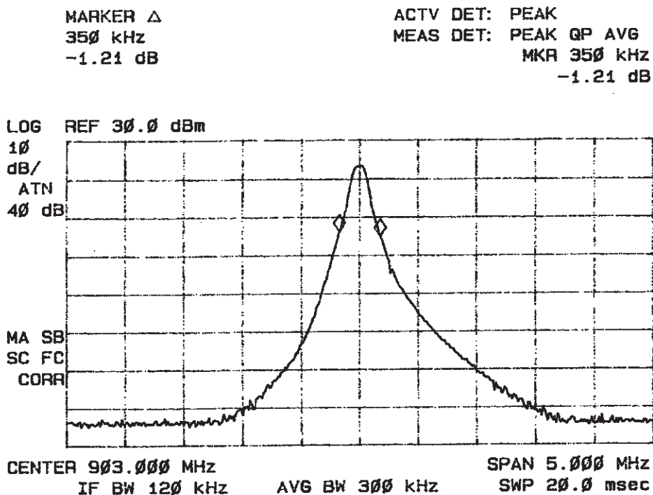
Figure 7 Occupied Bandwidth CW Mode 903 MHz
