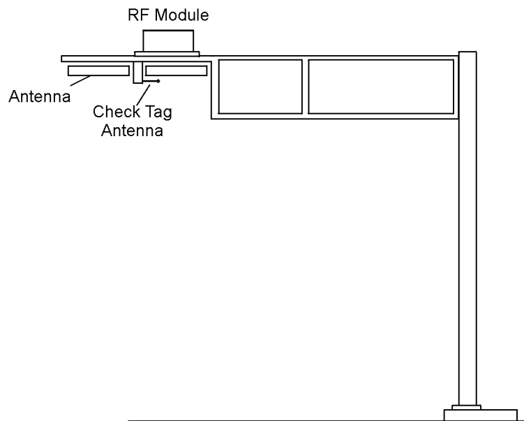
Figure 4-4 Cantilever Arm Mount (Bistatic Configuration)
