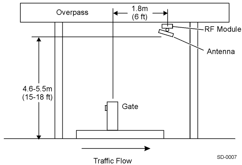
Figure 4-3 Overpass Mount
