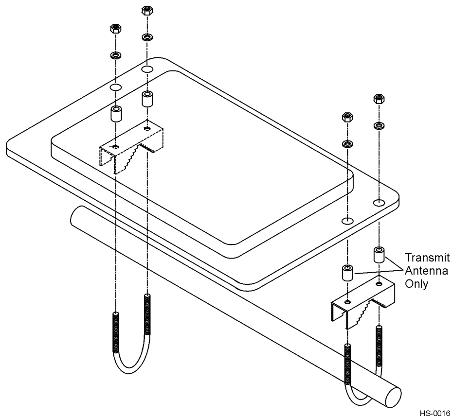
Figure 4-15 AA3152 UTA Mounting and Connections
