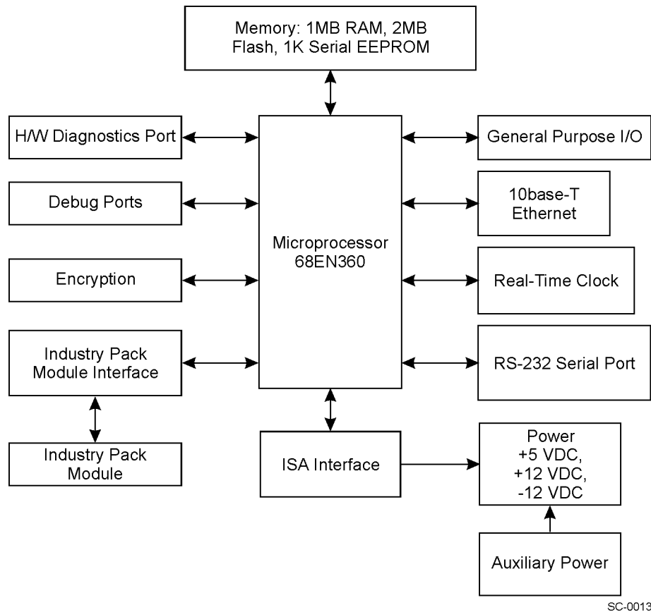
Figure B-3 IT2020 Reader Logic Card Functional Block Diagram
