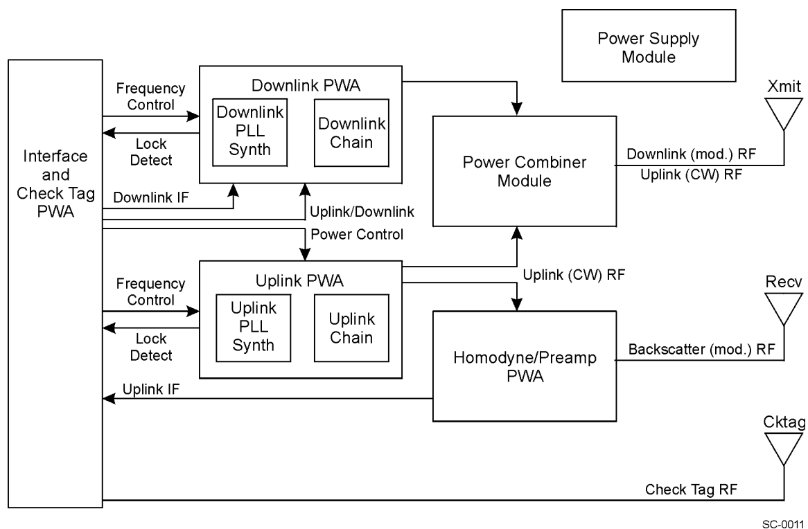
Figure B-7 IT2611 RF Module Functional Block Diagram (Bistatic Configuration)
