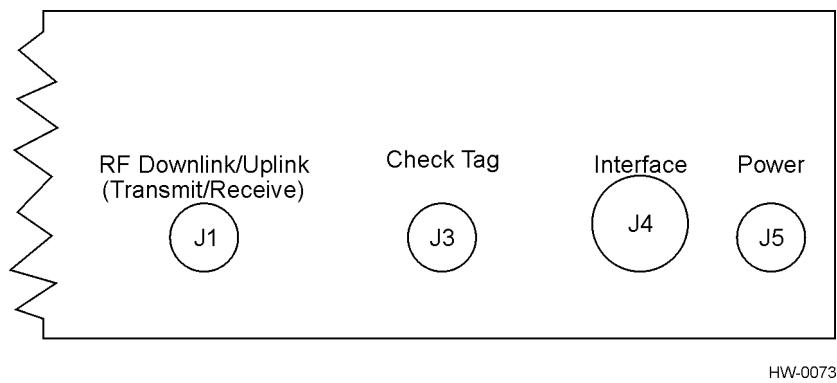
Figure D-5 Monostatic RF Module Interface
