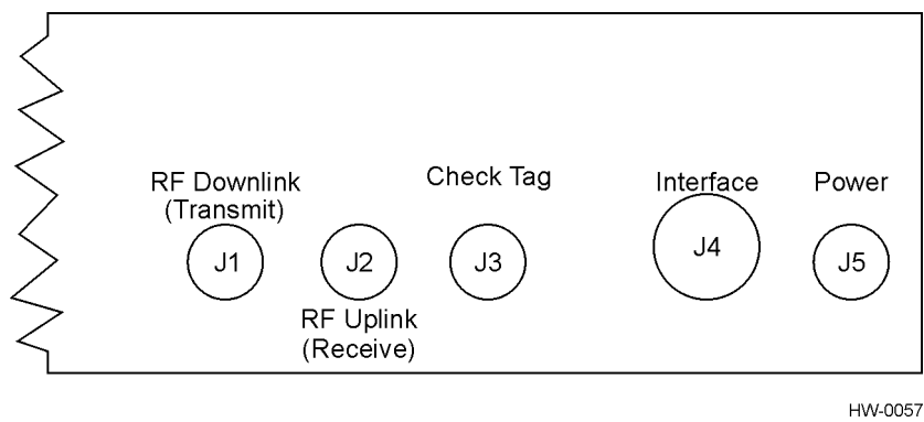
Figure D-4 Bistatic RF Module Interface
