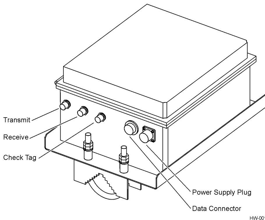
Figure 4-14 IT2611 RF Module Connectors (Monostatic RF Module Shown)
