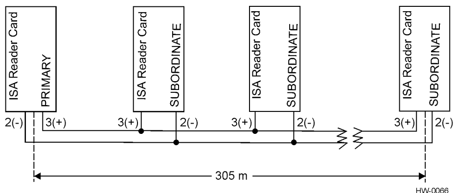
Figure D-2 Typical TDM Installation
