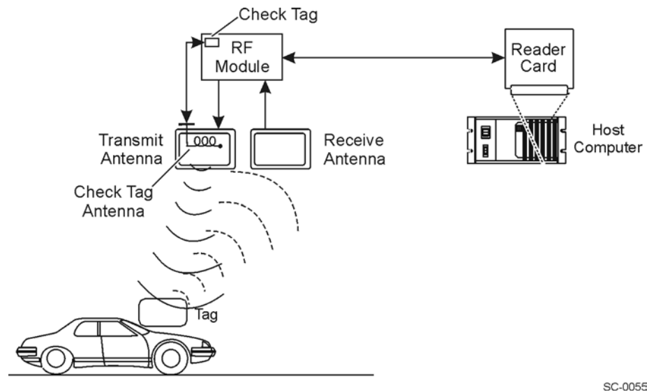
Figure 2-1 Typical RFID Components for a Bistatic (Two-Antenna) Configuration
