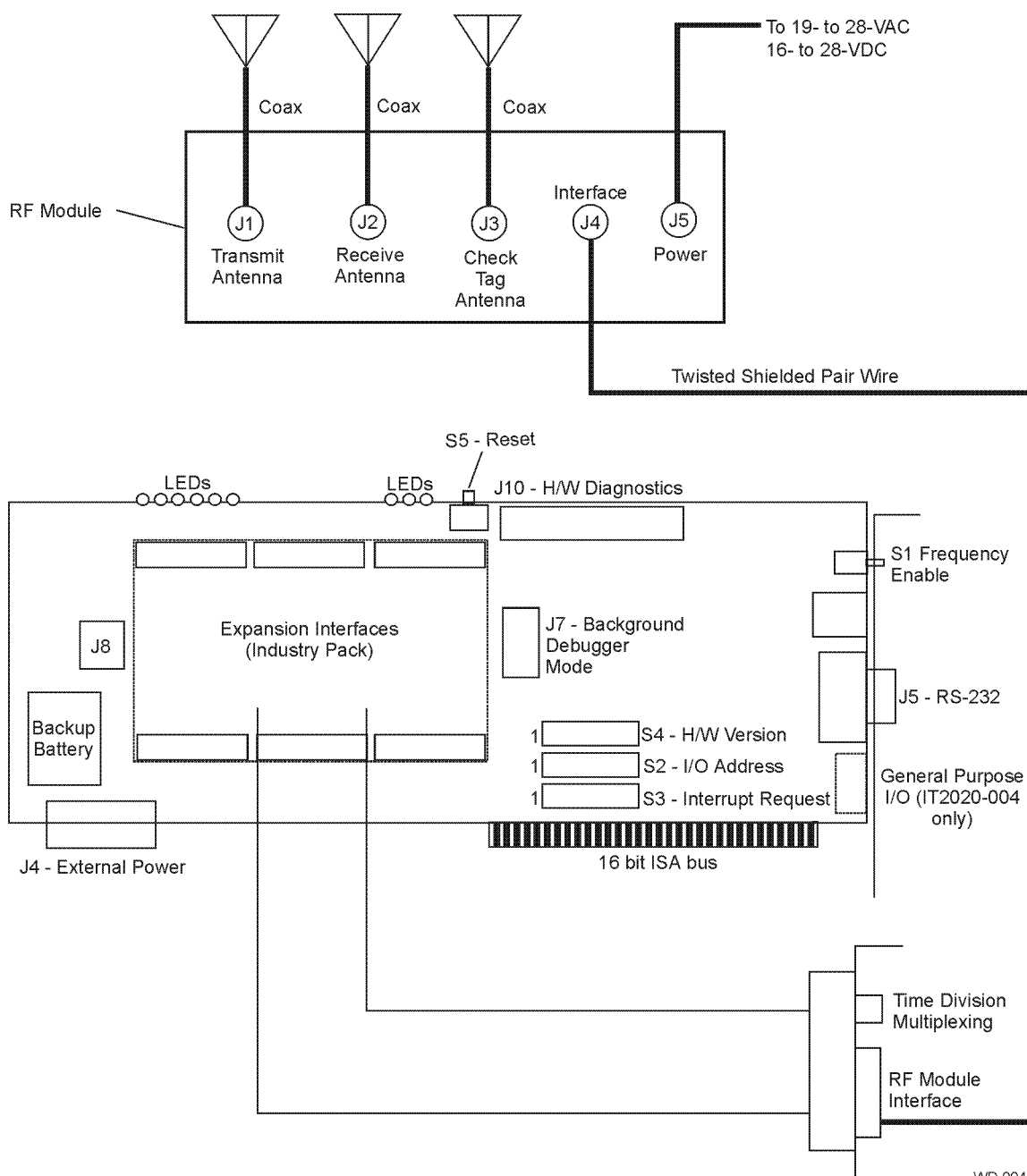
Figure B-5 Minimum Connections for the IT2020 Reader Logic Card Interface (Bistatic Application)
