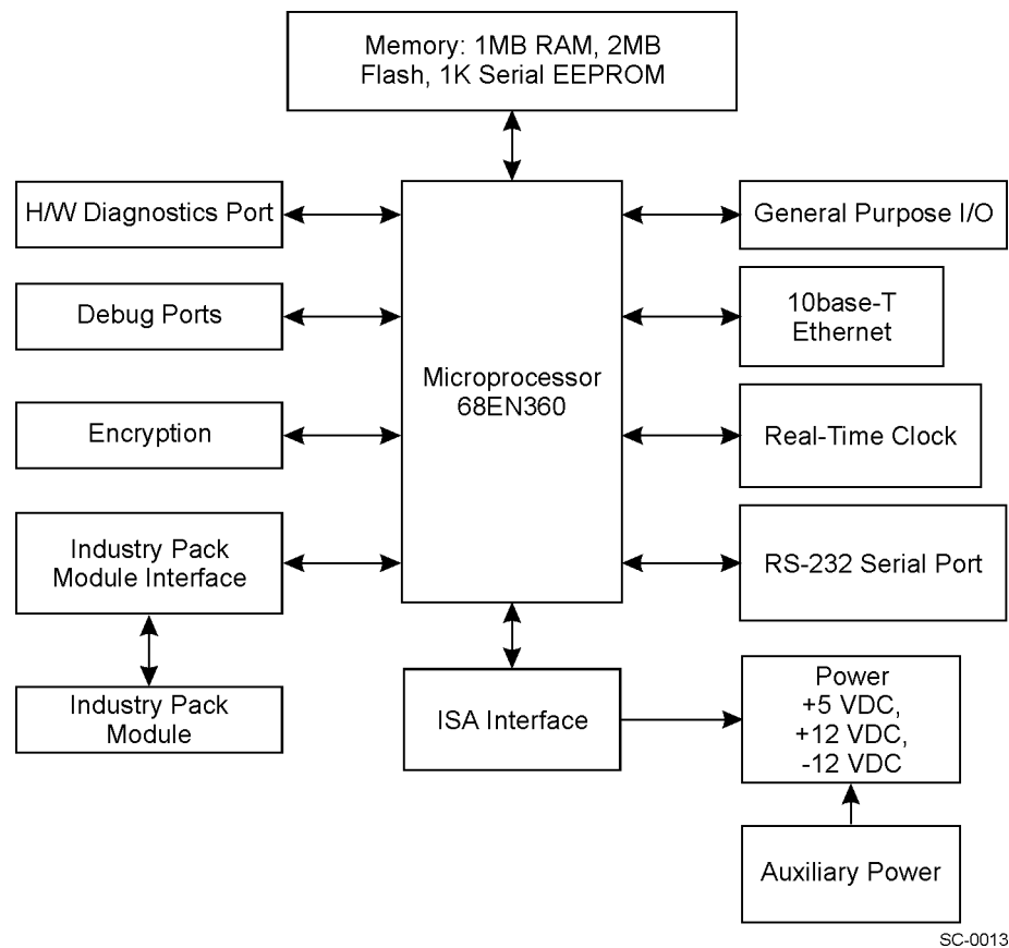
Figure 3-3 IT2020 Reader Logic Card Block Diagram
