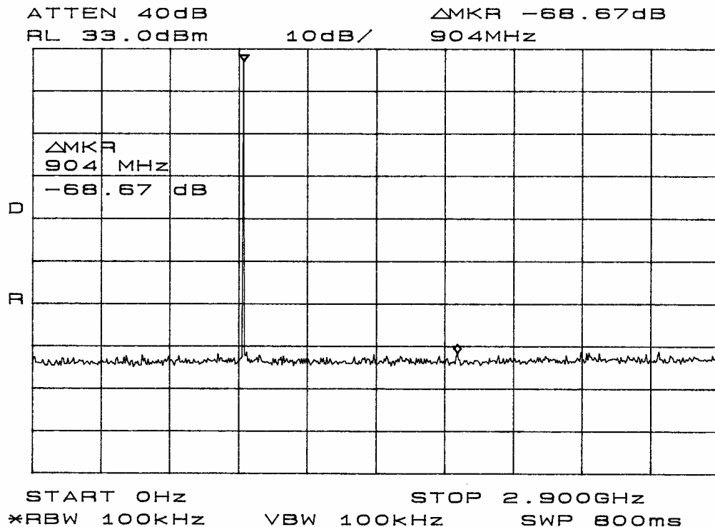
Figure 3 Emissions at Antenna Terminal
