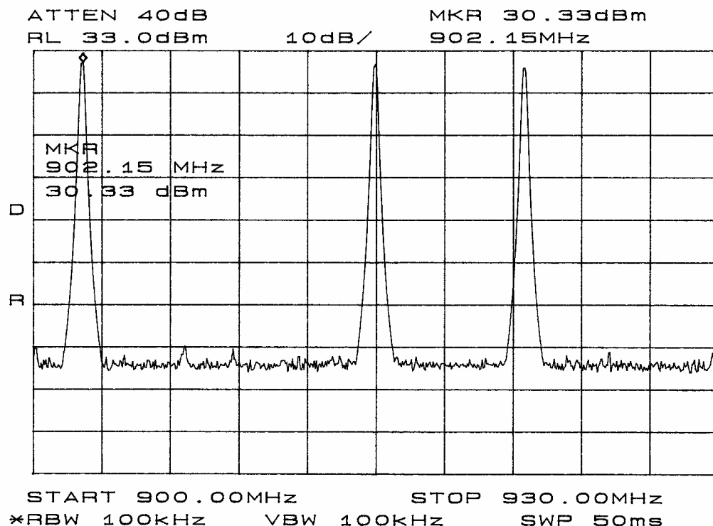
Figure 1 Power output.
