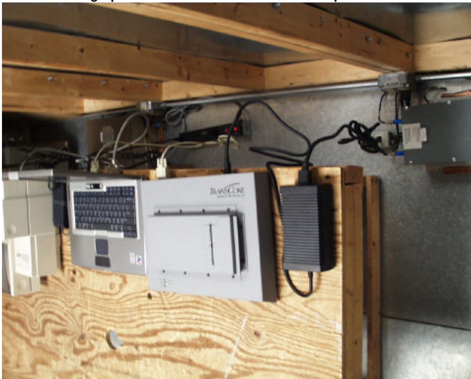
AP4118 Photographs of AC Line Conducted test setup.
