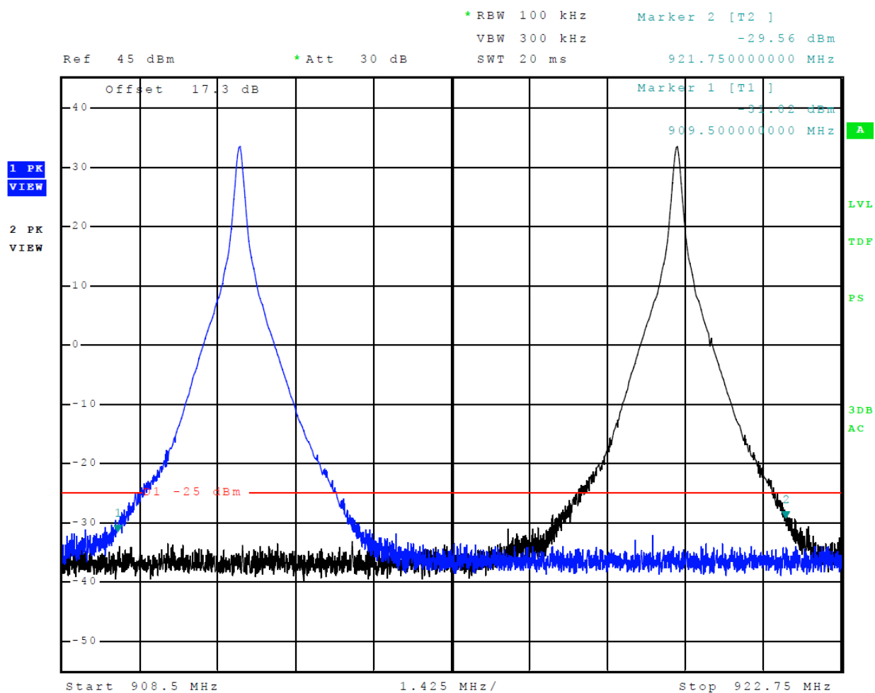
Figure 21 Emissions Mask EPC
