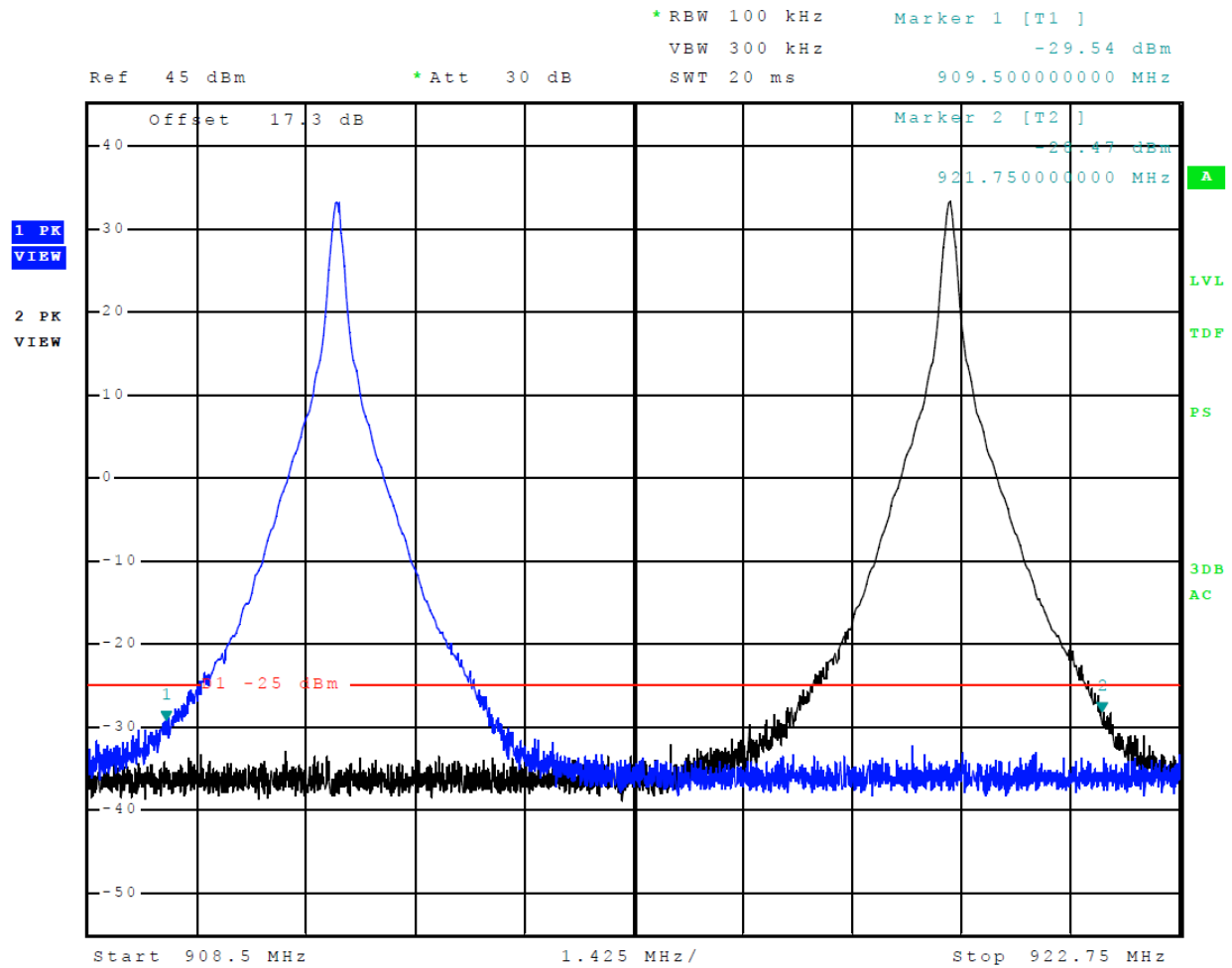
Figure 19 Emissions Mask SeGo
