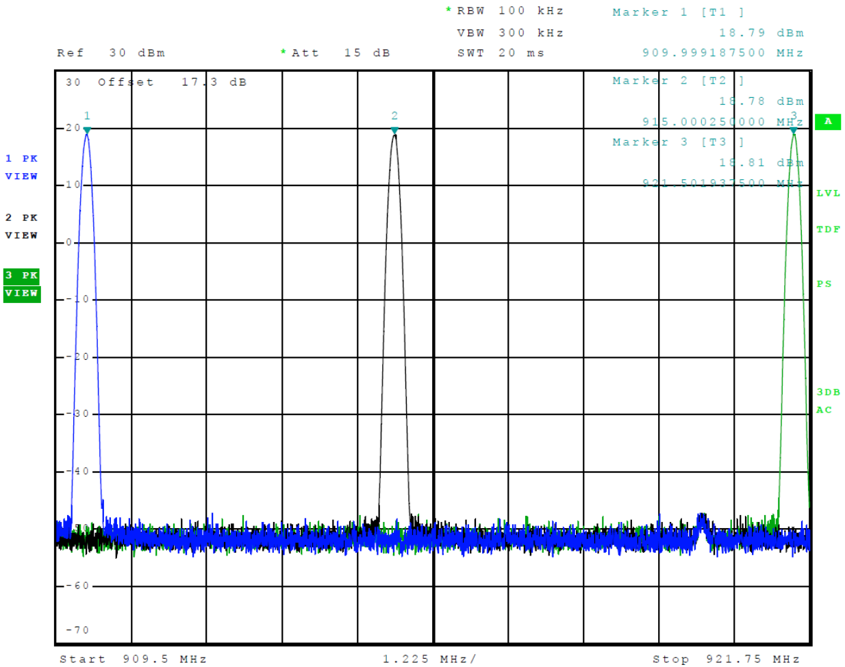
Figure 4 Transmitter Output Across Frequency Band CW (ATA) Lowest Power Level 910-921.75 MHz band
