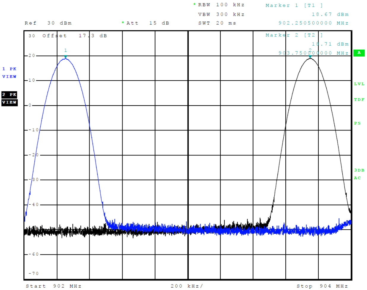
Figure 3 Transmitter Output Across Frequency Band CW (ATA) Lowest Power Level 902-904 MHz band
