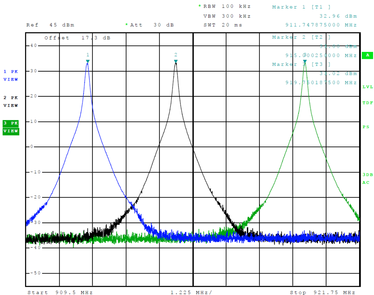
Figure 5 Transmitter Output Across Frequency Band eGo
