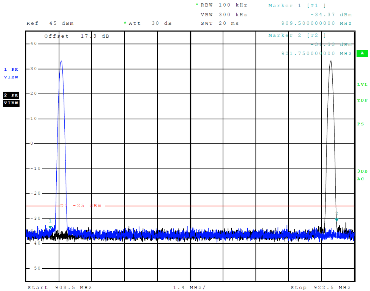
Figure 15 Emissions Mask ATA High Power (909.5-921.75 MHz Band)
