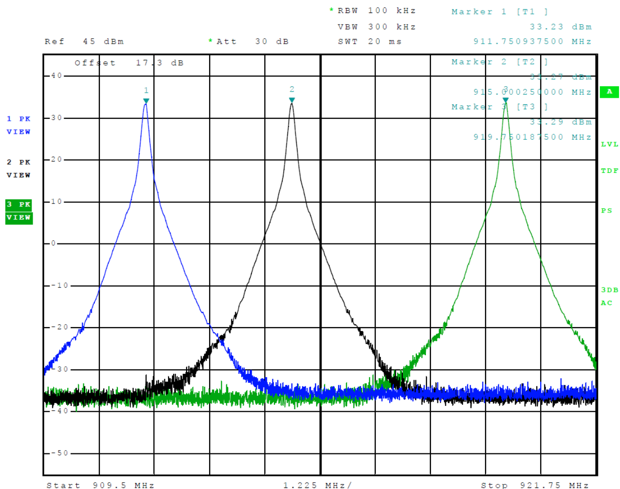
Figure 8 Transmitter Output Across Frequency Band EPC
