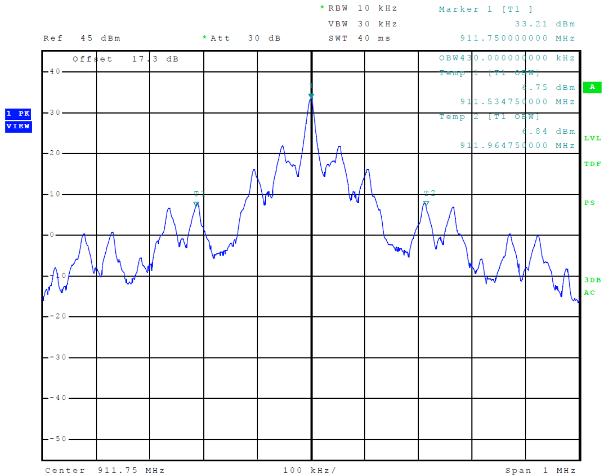
Figure 13 Occupied Bandwidth EPC
