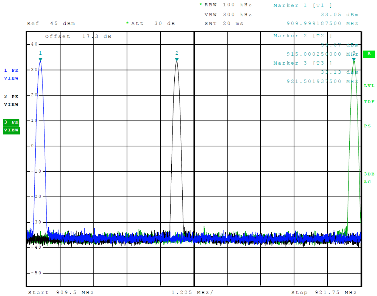
Figure 2 Transmitter Output Across Frequency Band CW (ATA) High Power Level 910-921.75 MHz band
