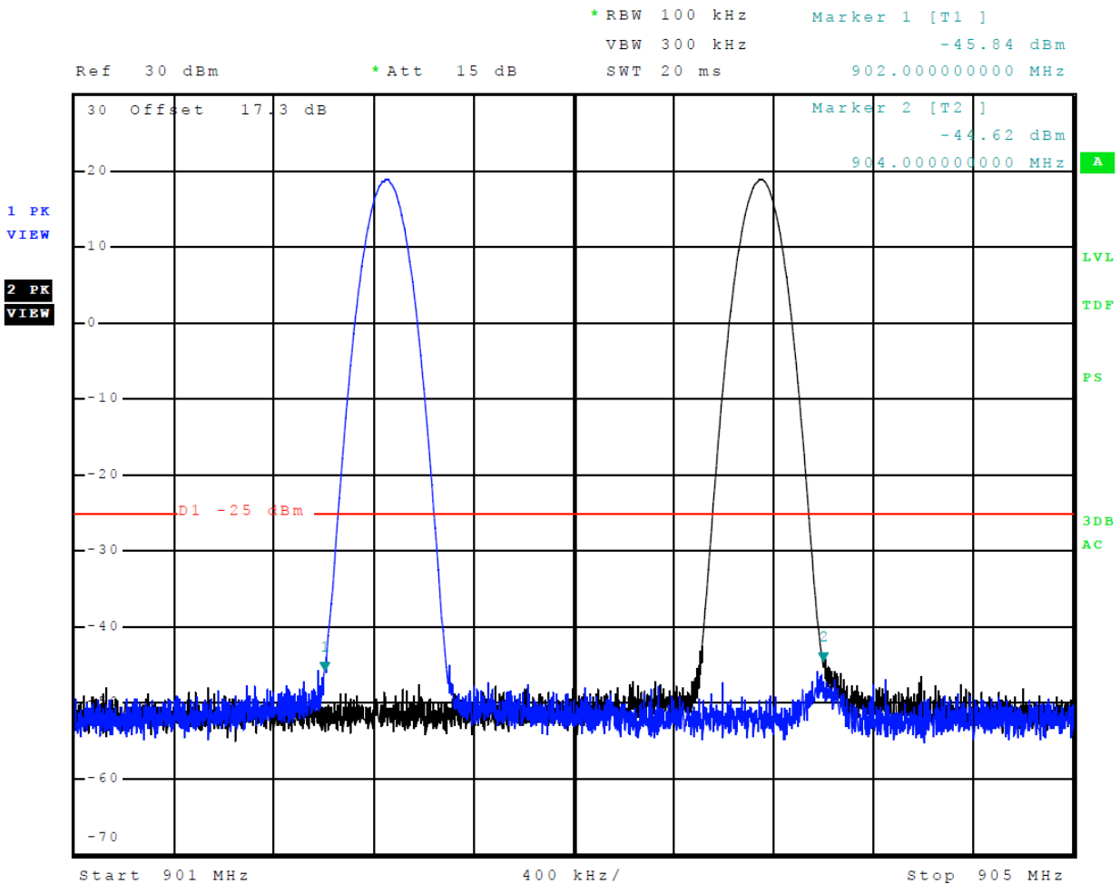
Figure 16 Emissions Mask ATA Low Power (902-904 MHz Band)
