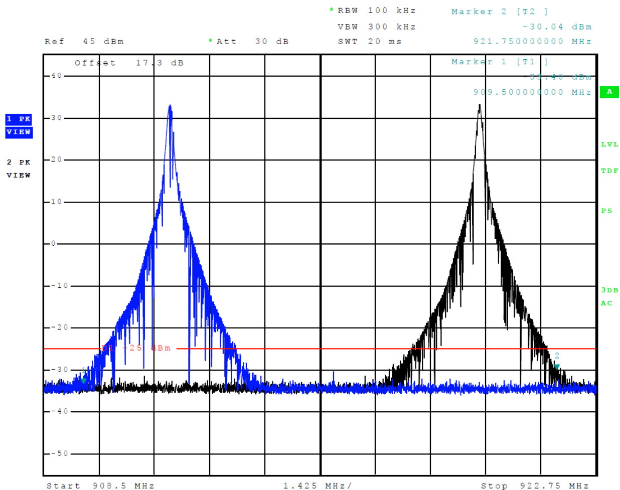
Figure 20 Emissions Mask IAG
