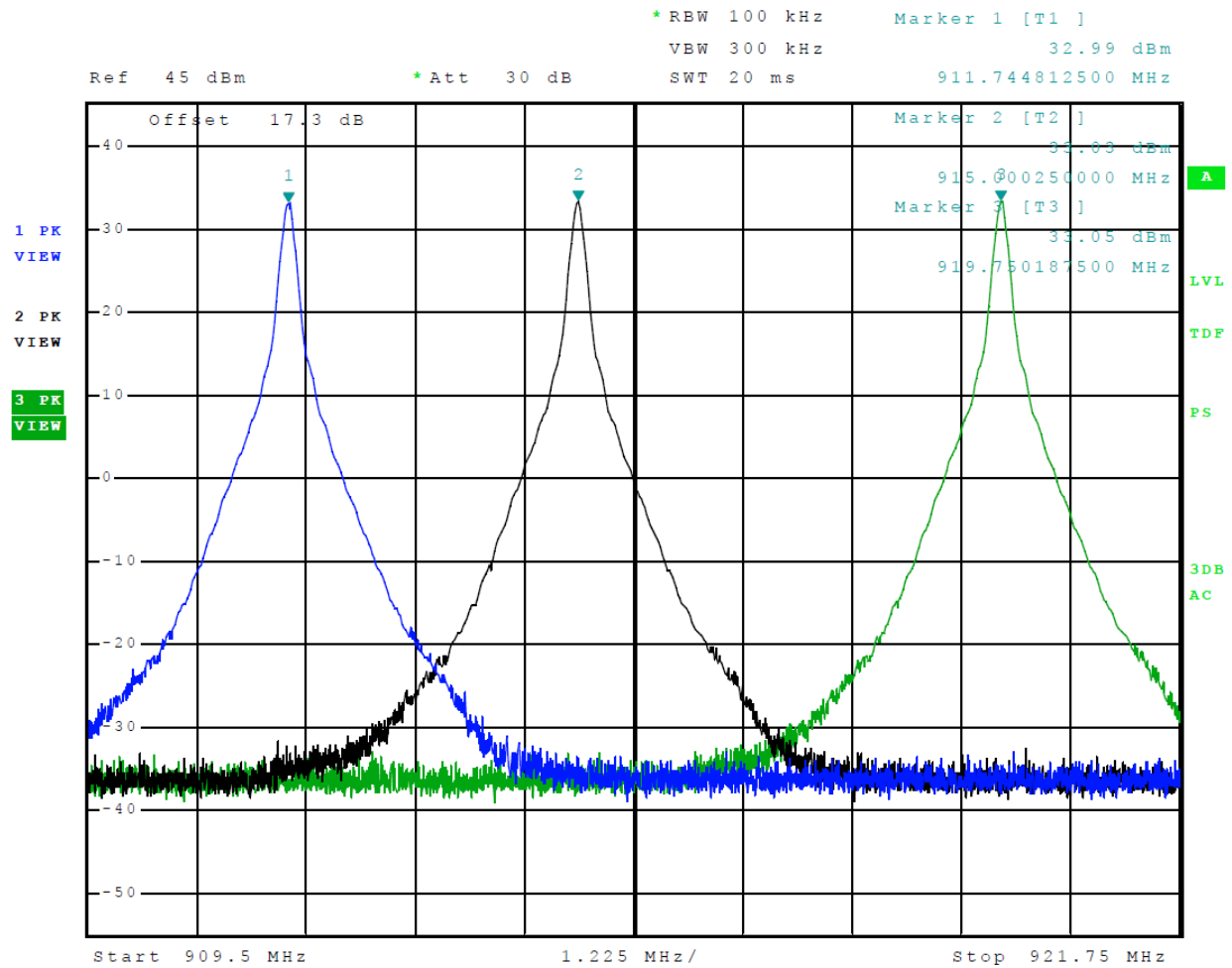
Figure 6 Transmitter Output Across Frequency Band SeGo
