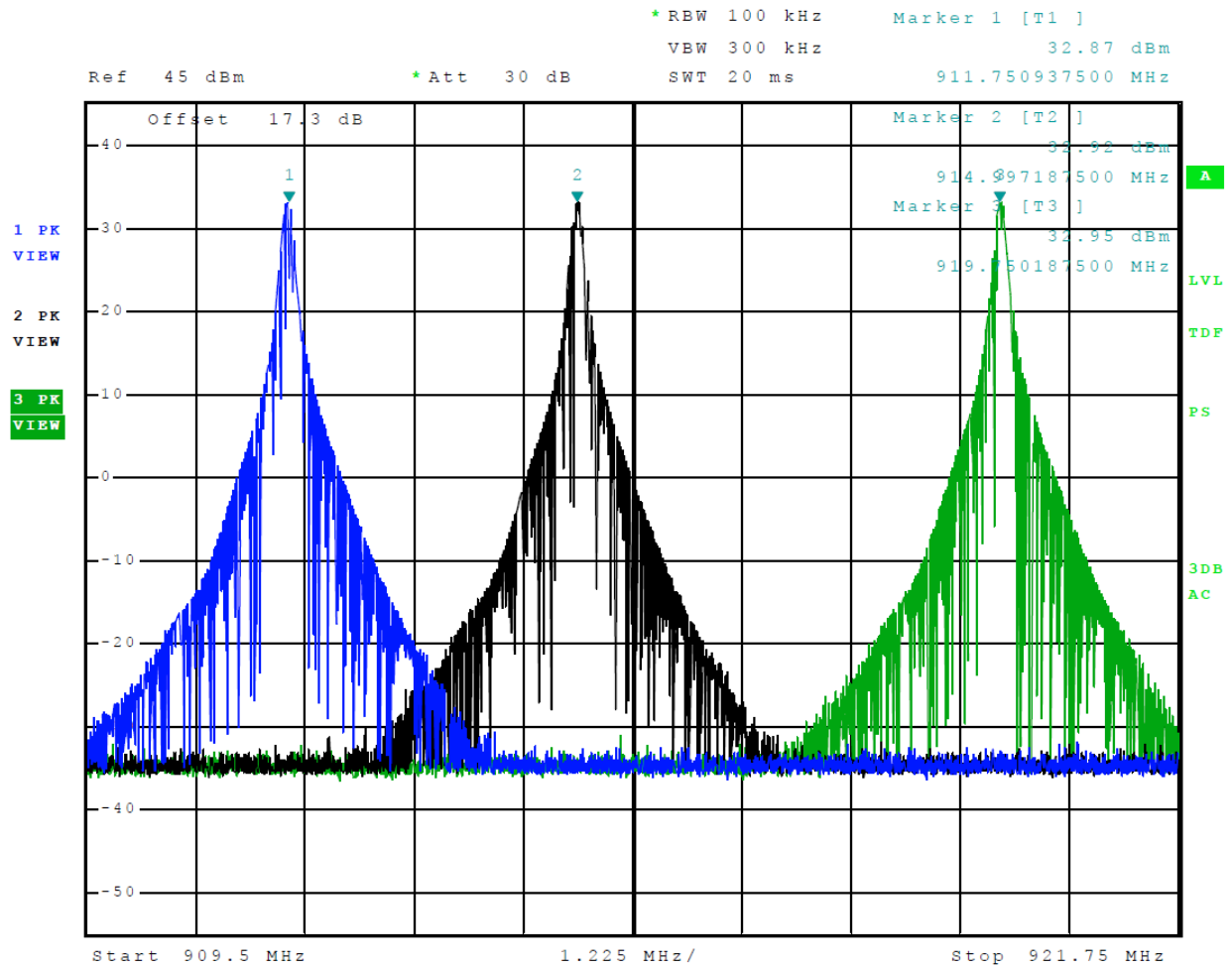
Figure 7 Transmitter Output Across Frequency Band IAG
