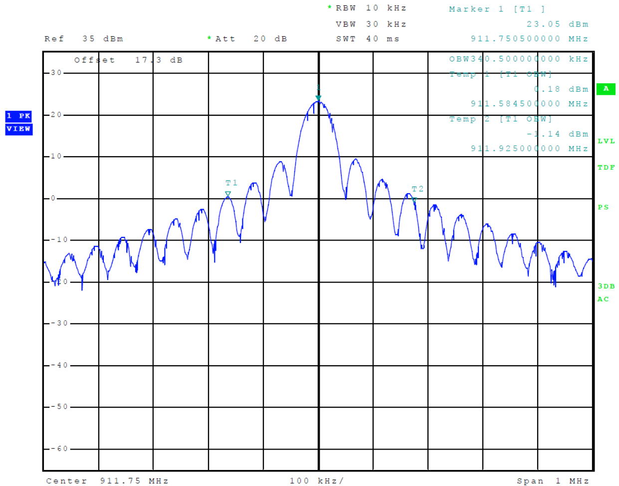
Figure 12 Occupied Bandwidth IAG
