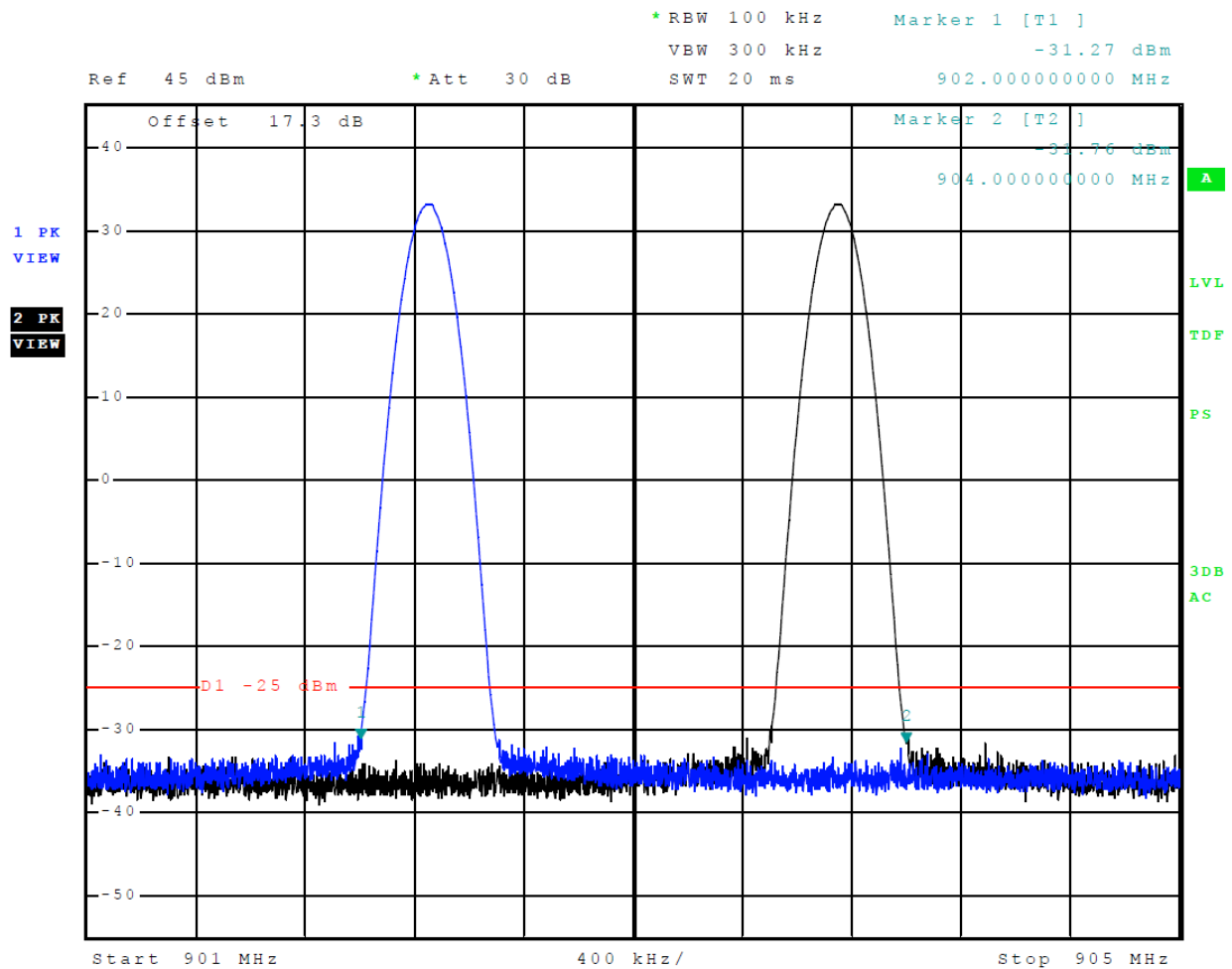
Figure 14 Emissions Mask ATA High Power (902-904 MHz Band)
