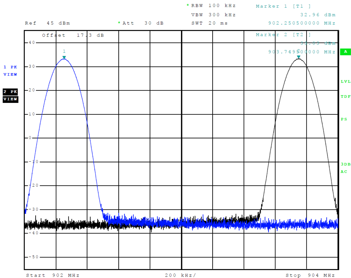
Figure 1 Transmitter Output Across Frequency Band CW (ATA) High Power Level 902-904 MHz band
