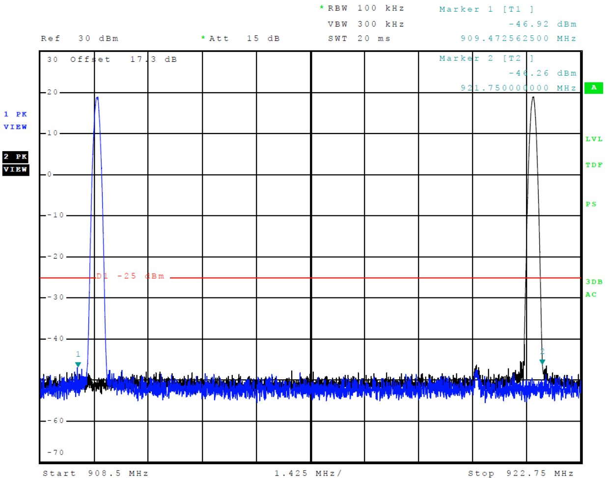
Figure 17 Emissions Mask ATA Low Power (909.5-921.75 MHz Band)
