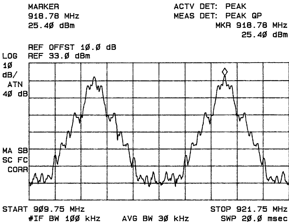
Figure 7 Emissions Mask
