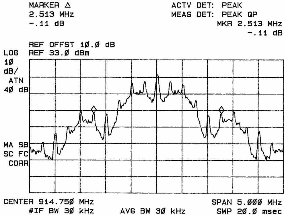
Figure two Occupied Bandwidth C-Vision Mode.
