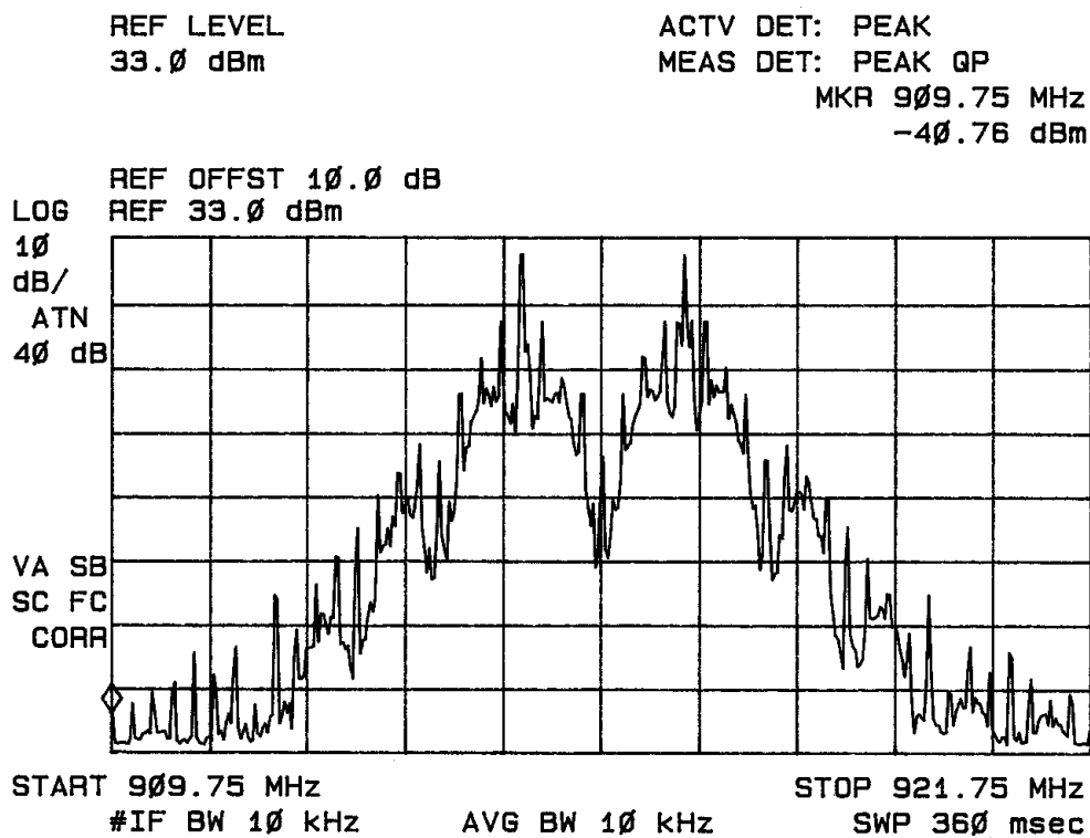
Figure 7 Emissions Mask
