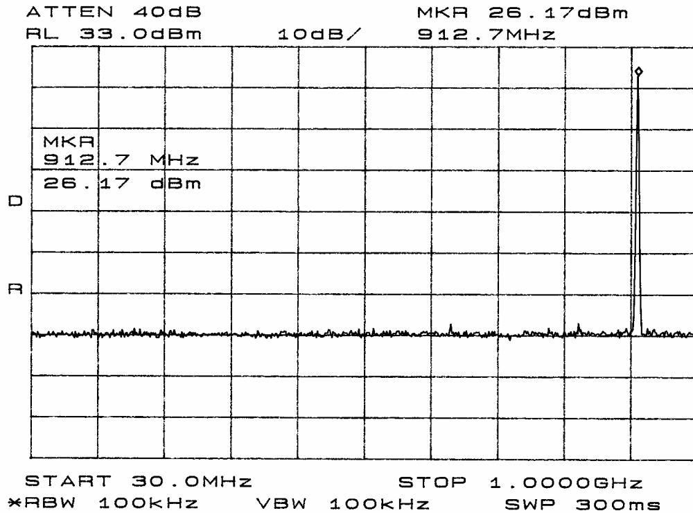
Figure 3 Spurious Emissions at Antenna Terminal
