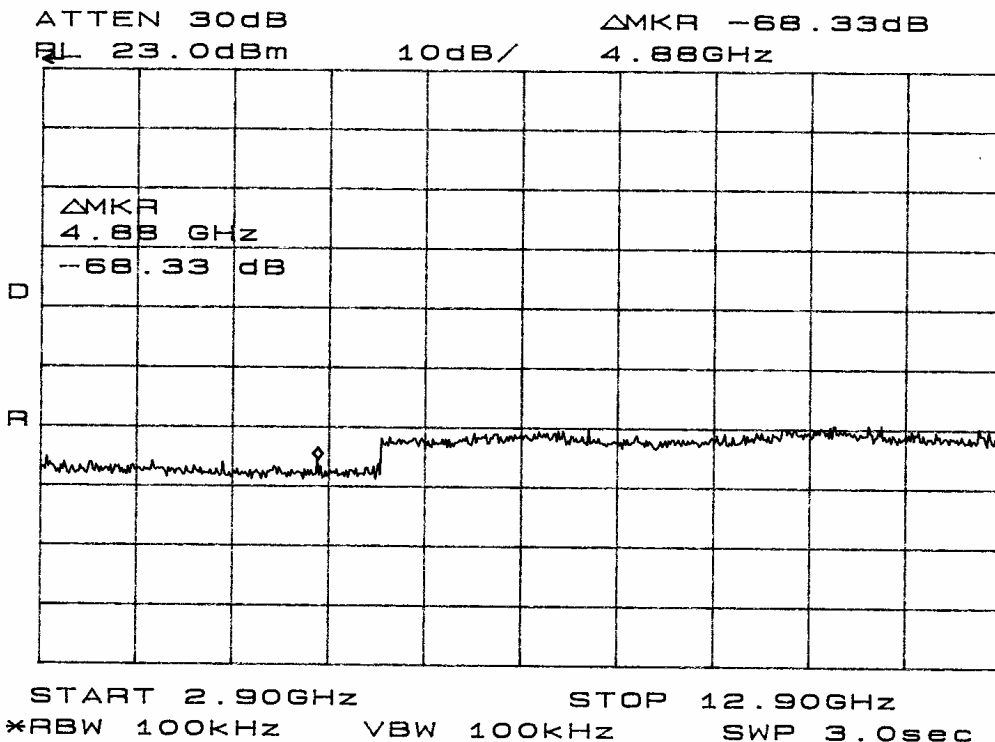
Figure 5 Spurious Emissions at Antenna Terminal
