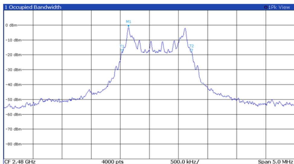
Figure: Plot of 99% Occupied Bandwidth Mode 3A, BT BLE (GMSK)
