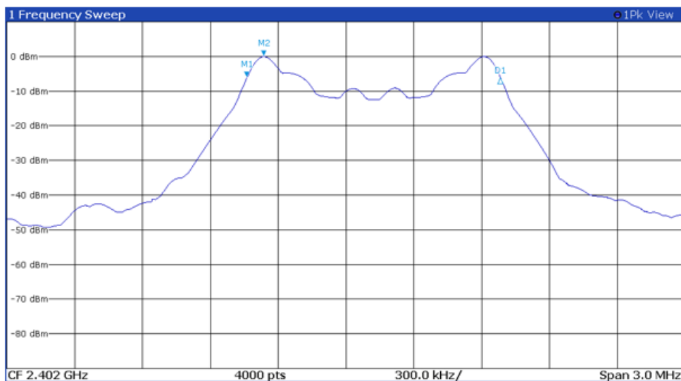
Figure: Plot of 6-dB Occupied Bandwidth Mode 3A, BT BLE (GMSK)
