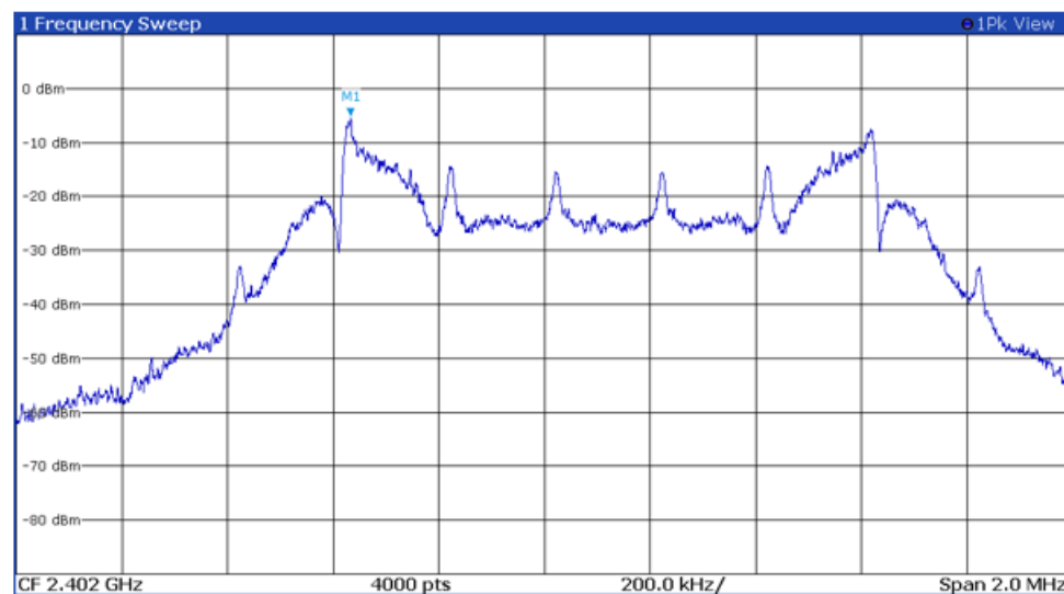
Figure: Plot of Transmitter Power Spectral Density Mode 3A, BT BLE (GMSK)
