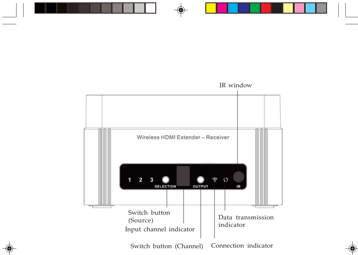
Figure 3: Receiver (RX) - front side
