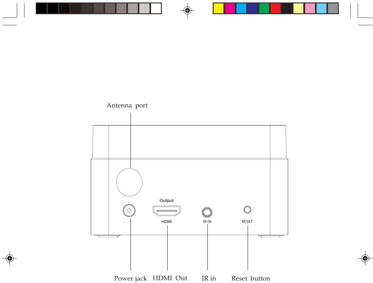
Figure 4: Receiver (RX) - rear side
