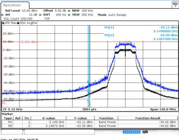
BE-R-LOW, MIMO-B, 802.11n20-HT8, Ch36
