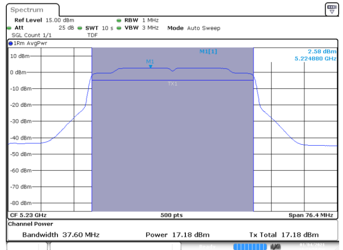
MIMO B-802.11ax-40MHz-Ch46-5230MHz-HE0
