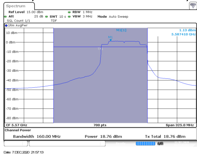
Channel 114
