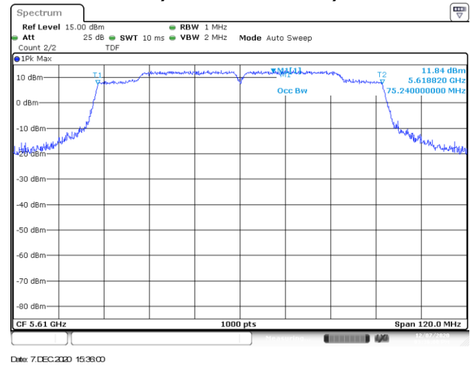
Channel 122
