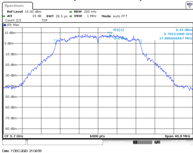
Channel 140
