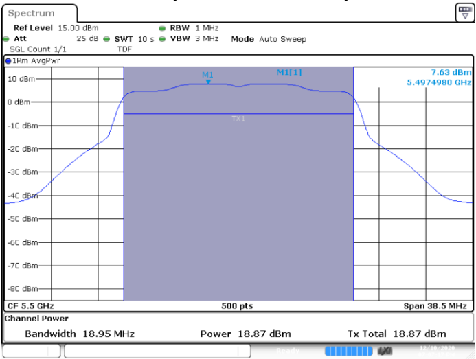
Channel 100
