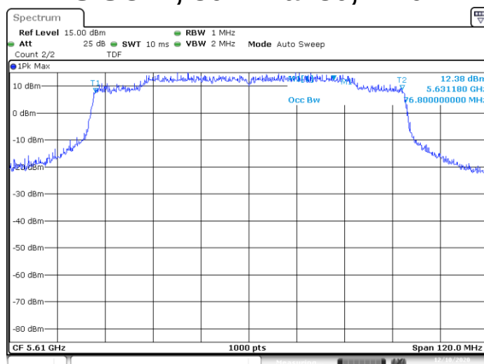
Channel 122
