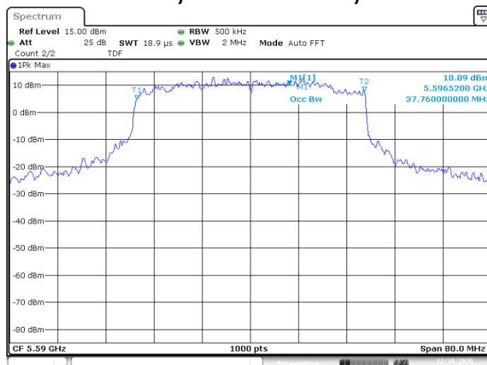
Channel 118
