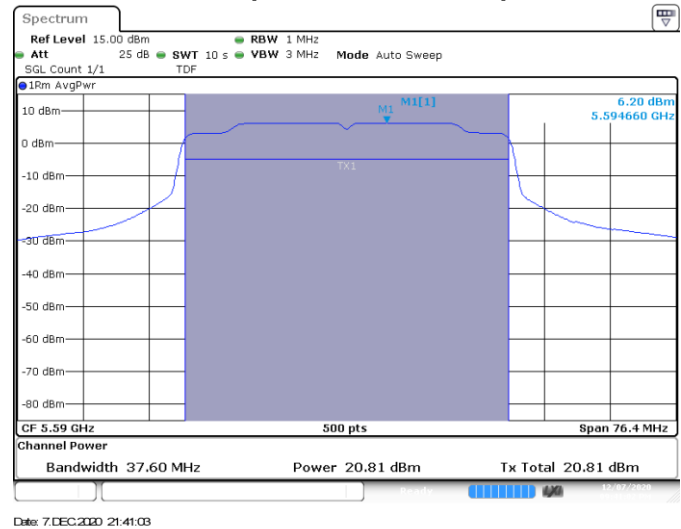
Channel 118
