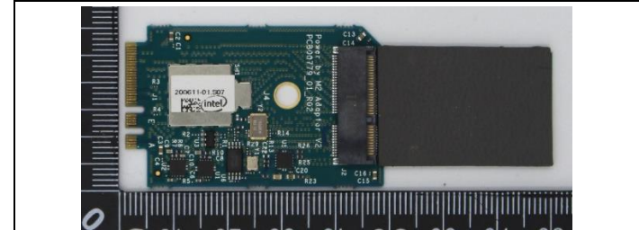
Extender board
