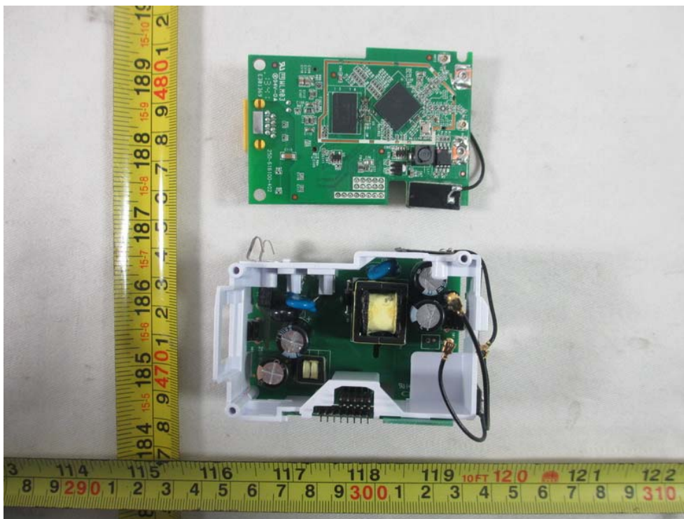
main board
