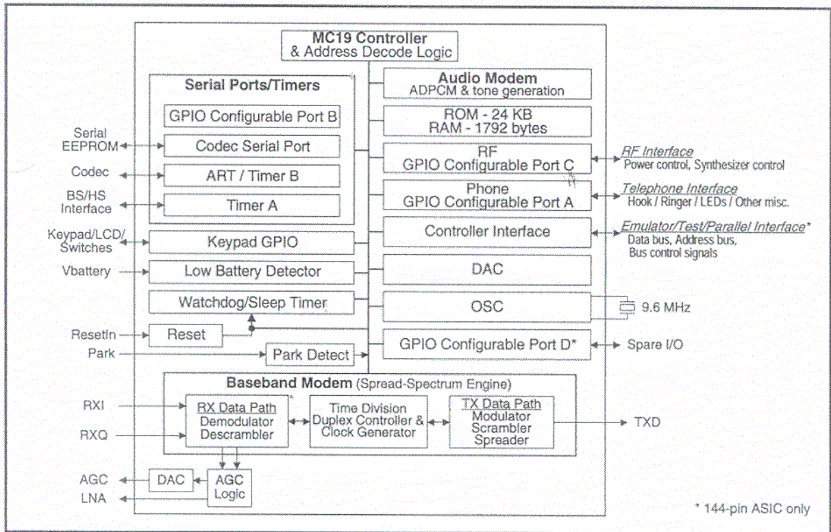
CR-201 ASIC Block Diagram
