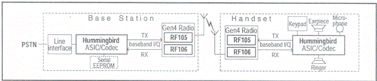
CR-201 Spread Spectrum Telephone System Architecture
