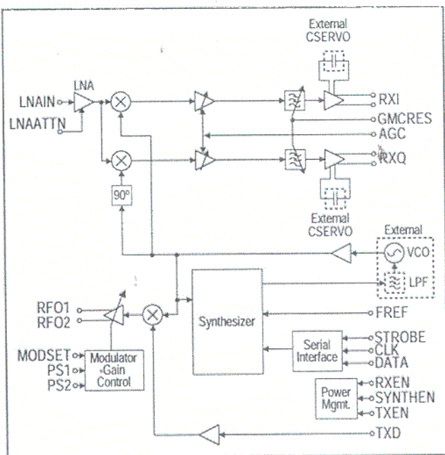
CR-201 RF Block Diagram
