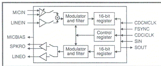
CR-201 CODEC Block Diagram
