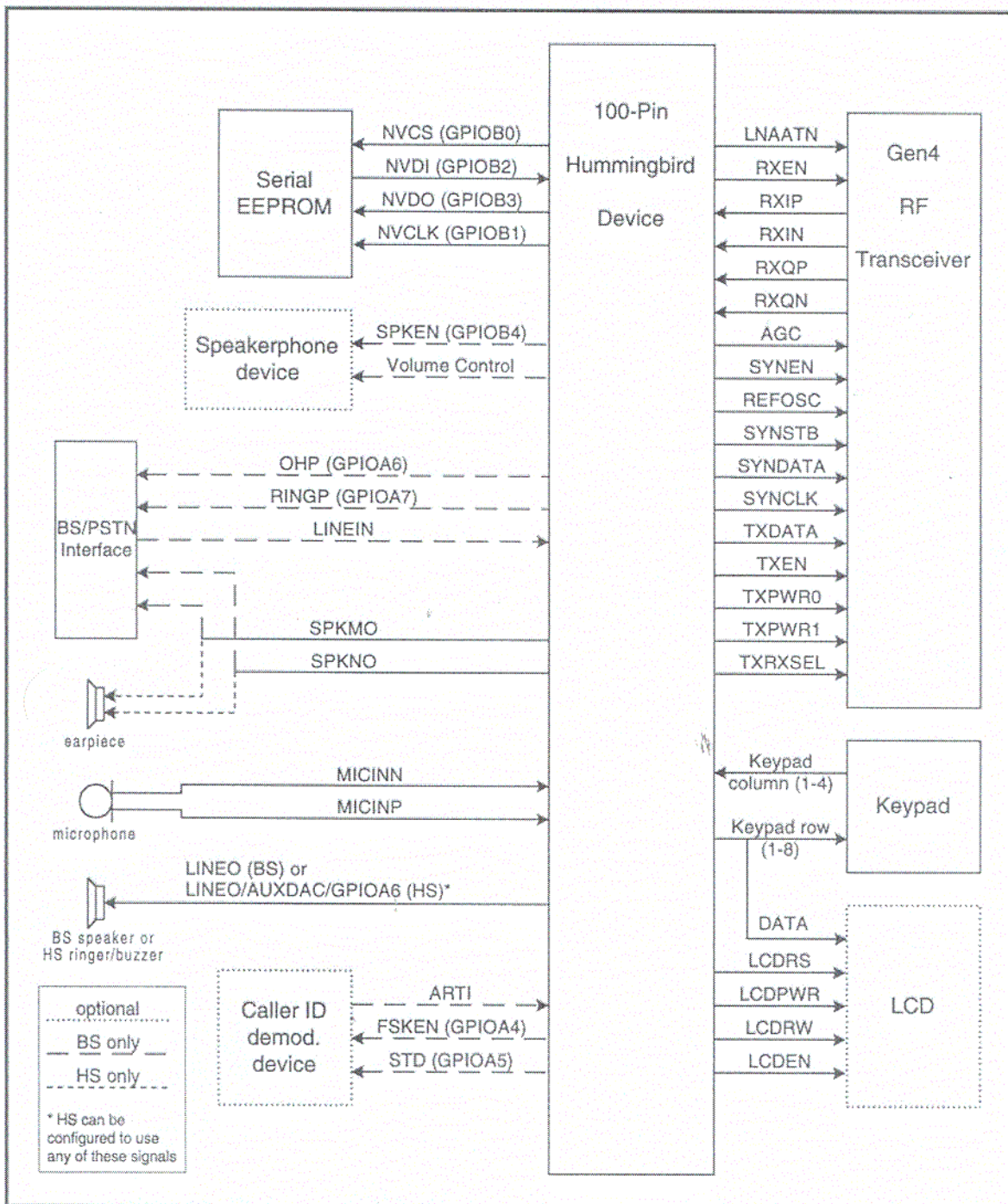
CR-201 System Block Diagram
