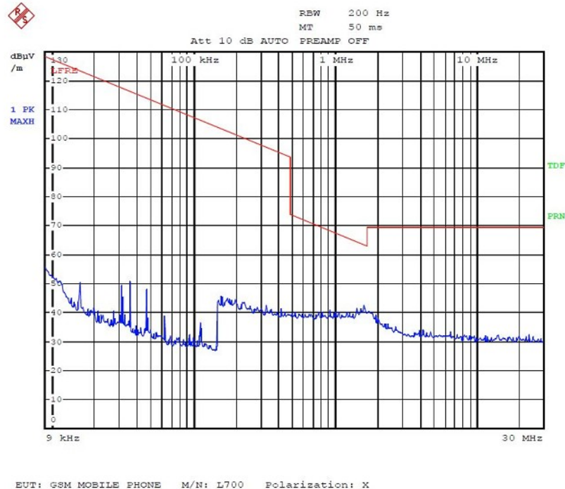
Radiated Emission Plot between 9 kHz ~ 30MHz
