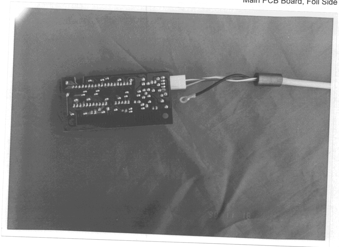
Figure 6 Main PCB Board, Foil Side
