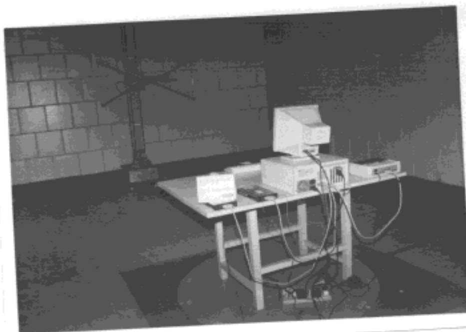
BACK VIEW OF RADIATED MEASUREMENT
